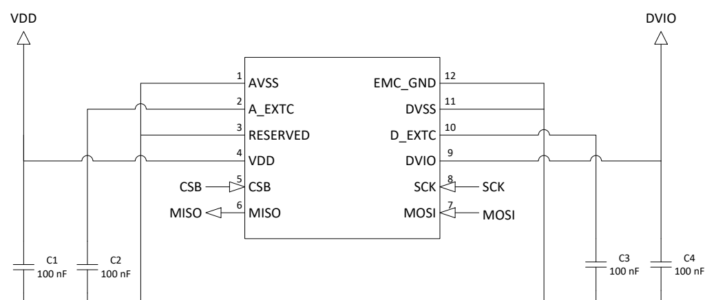
Figure 16 Application schematic.
