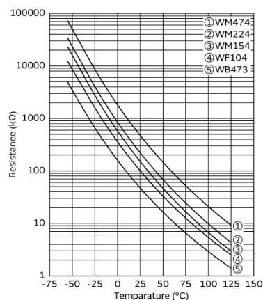
Resistance-Temperature Characteristics
