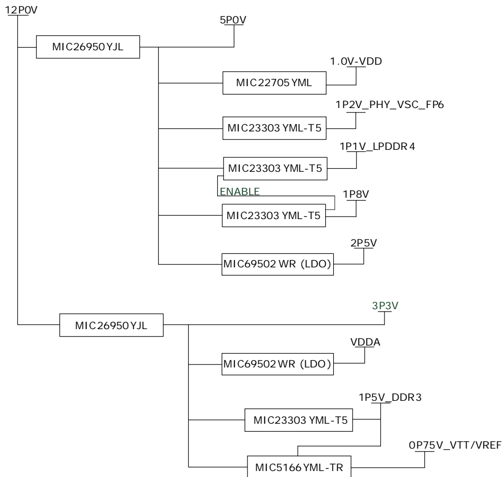
Figure 3 • Voltage Rails on PolarFire SoC ICICLE Kit
