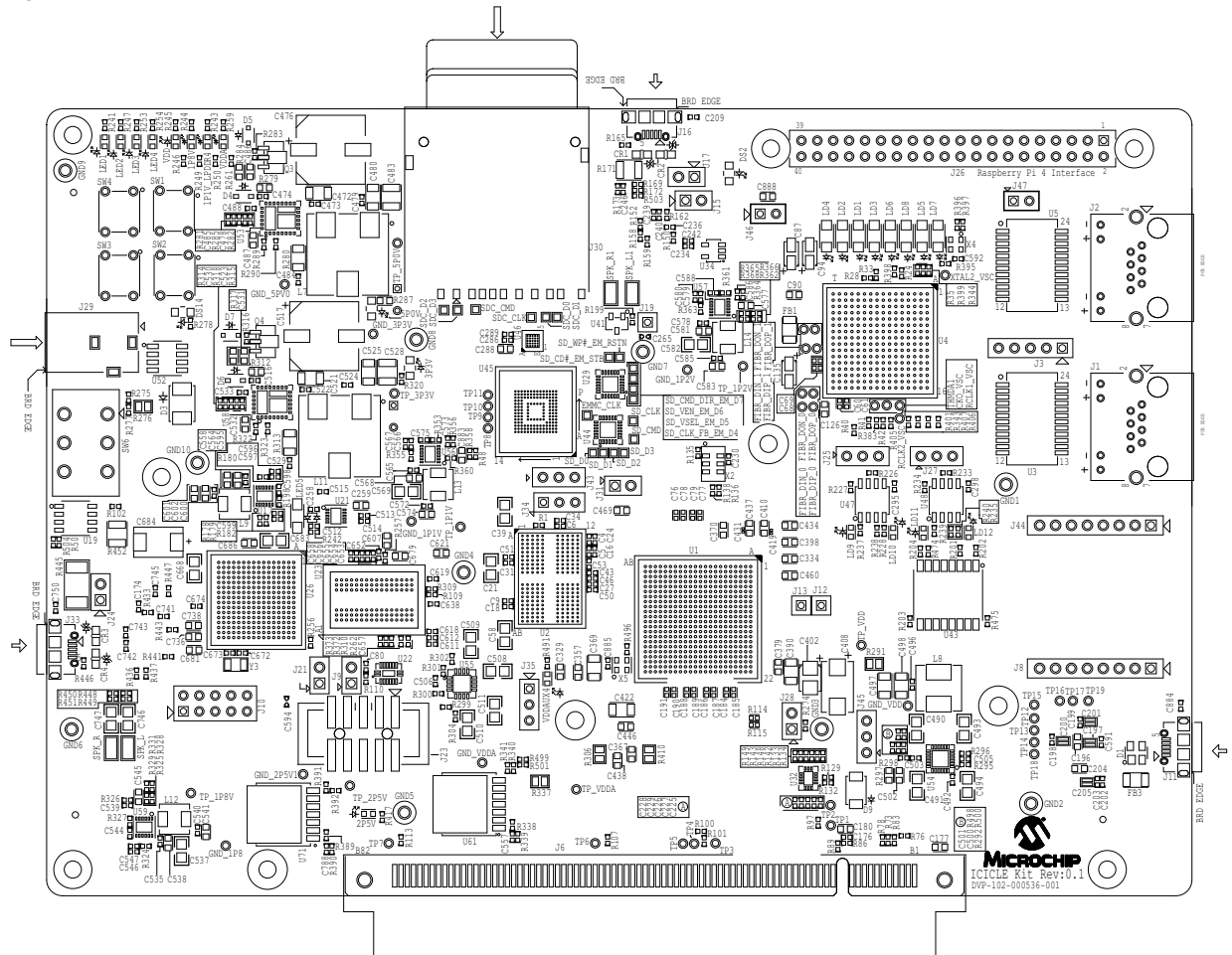
Figure 8 • Silkscreen Top View
