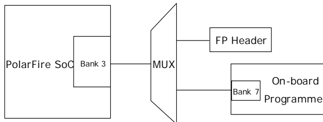
Figure 5 • PolarFire SoC Programming Scheme Block Diagram
