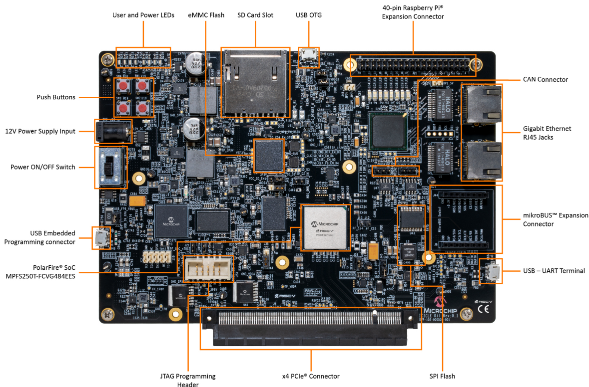
Figure 2 • PolarFire SoC ICICLE Kit
