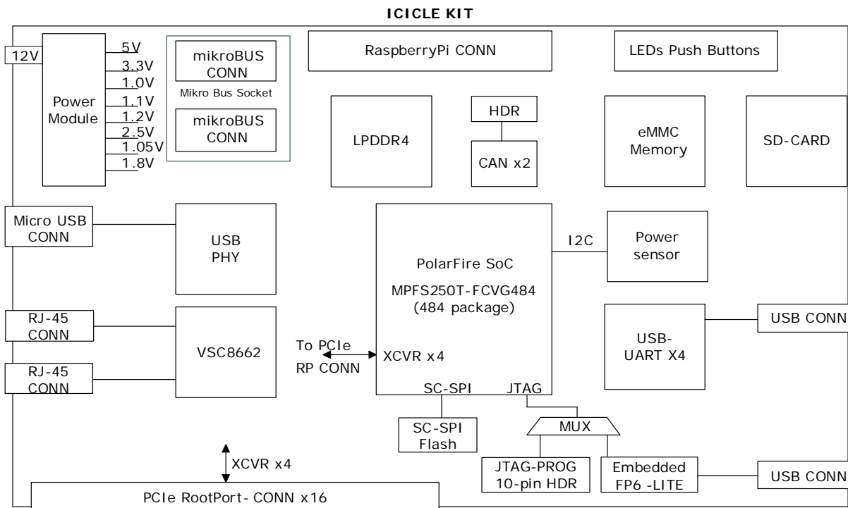
Figure 1 • PolarFire SoC ICICLE Kit Block Diagram
