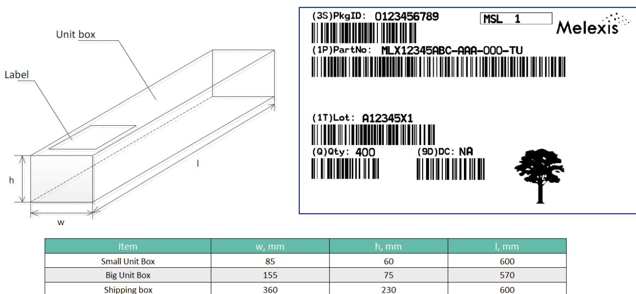
Figure 36 – Box for tubes – 11 tubes or less per box (small or big)
