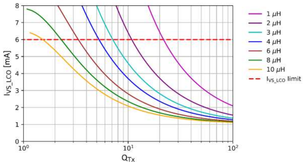
Figure 5 – I_{V_S\text{LCO}} as function of Q_{\text{Tx}} for LCO frequency of 3.5 MHz
