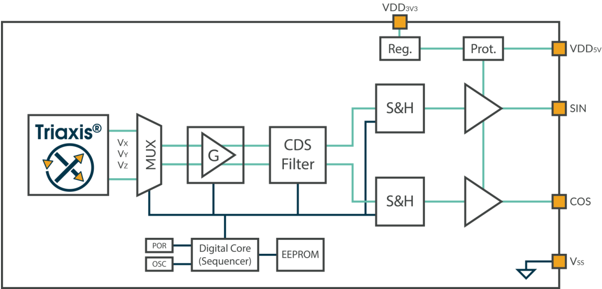
Figure 3: Functional Diagram
