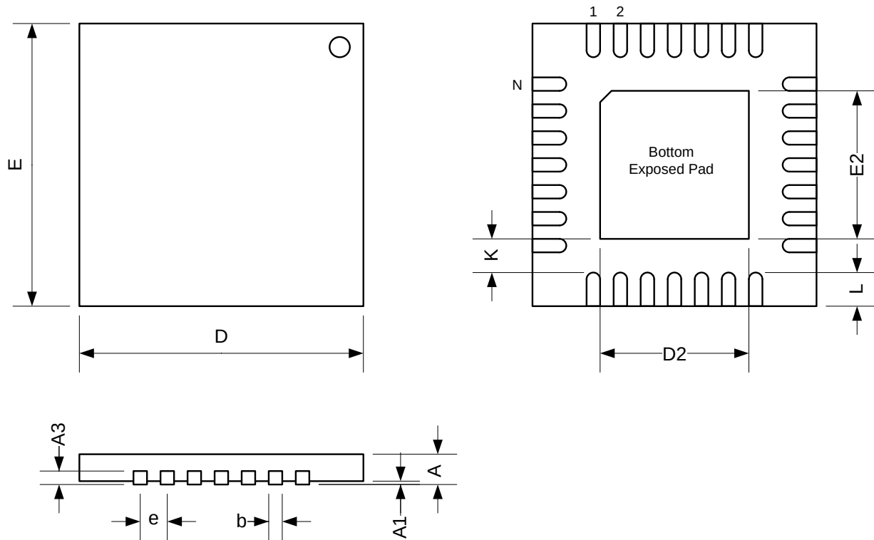
Figure 33 - QFN28 Drawing
