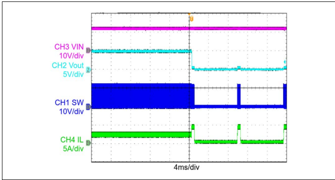
Figure 19: Short Circuit Protection— V_{IN} = 12V , V_{OUT} = 5V , I_{OUT} = 2A —Short
