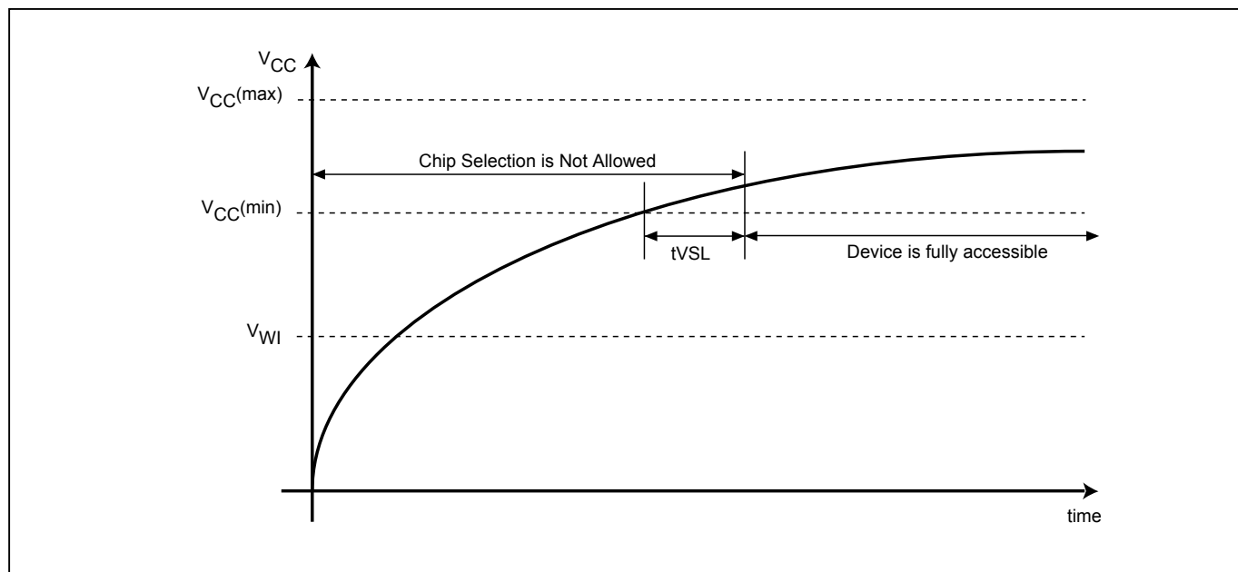
Figure 47. Power-up Timing
