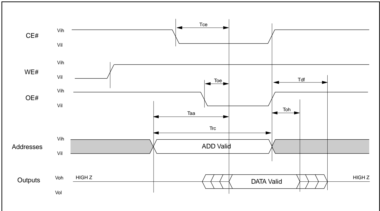
Figure 2. READTIMING WAVEFORMS
