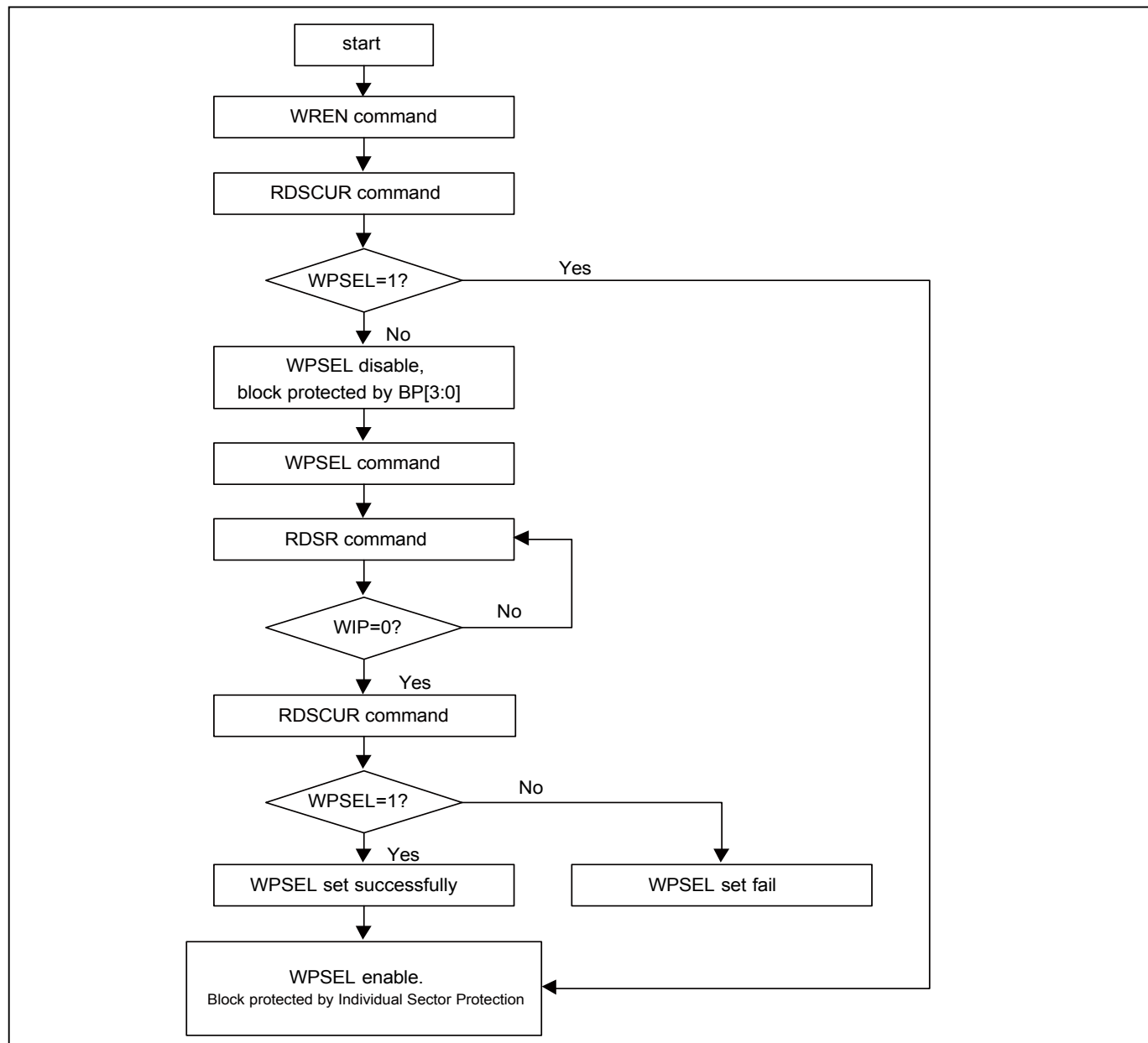
Figure 70. WPSEL Flow
