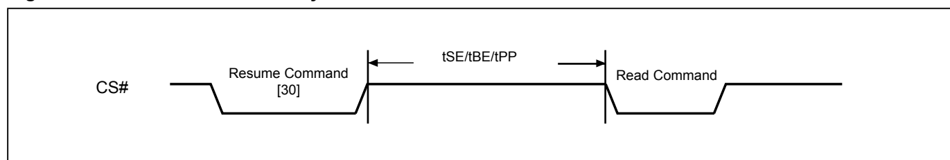
Figure 80. Resume to Read Latency
