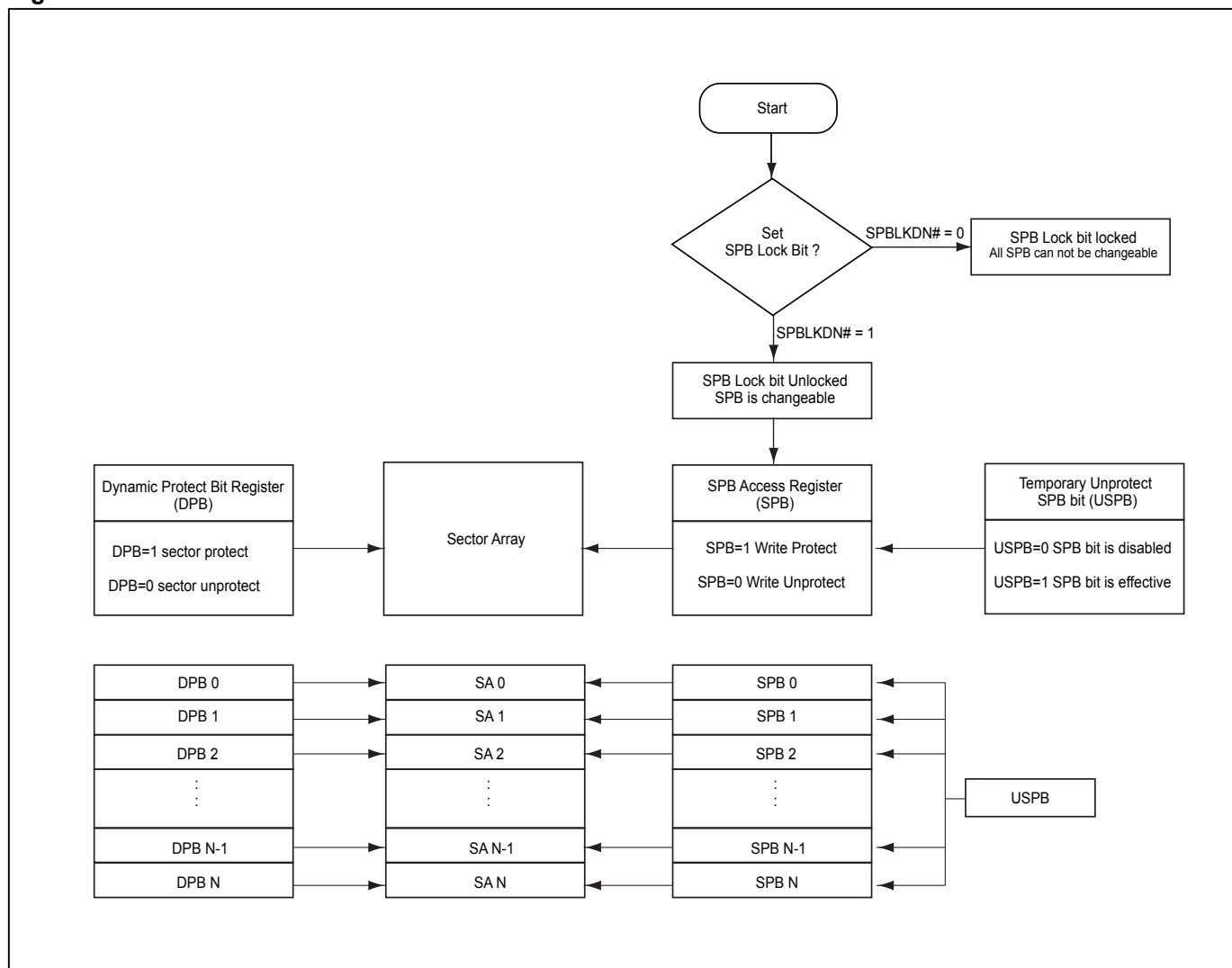
Figure 70. Advanced Sector Protection Overview
