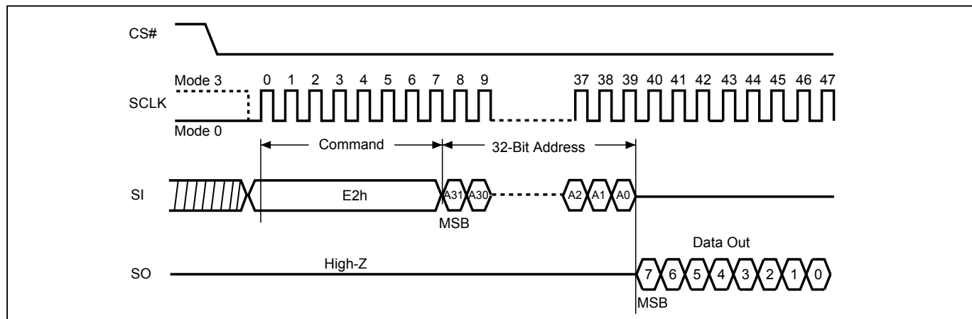
Figure 73. Read SPB Status (RDSPB) Sequence
