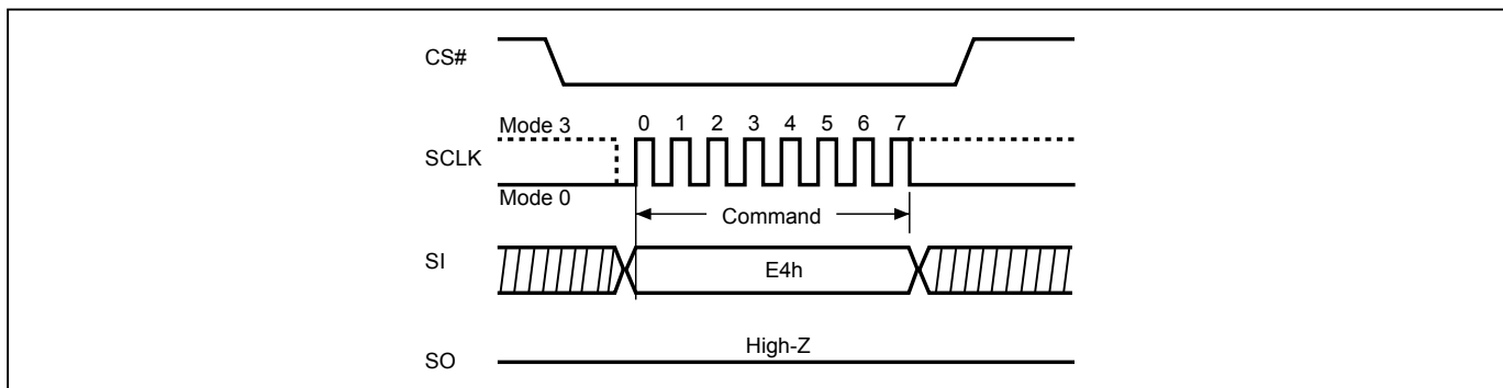
Figure 74. SPB Erase (ESSPB) Sequence
