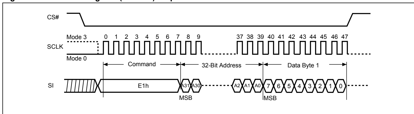
Figure 77. Write DPB Register (WRDPB) Sequence
