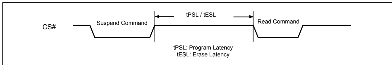
Figure 78. Suspend to Read Latency
