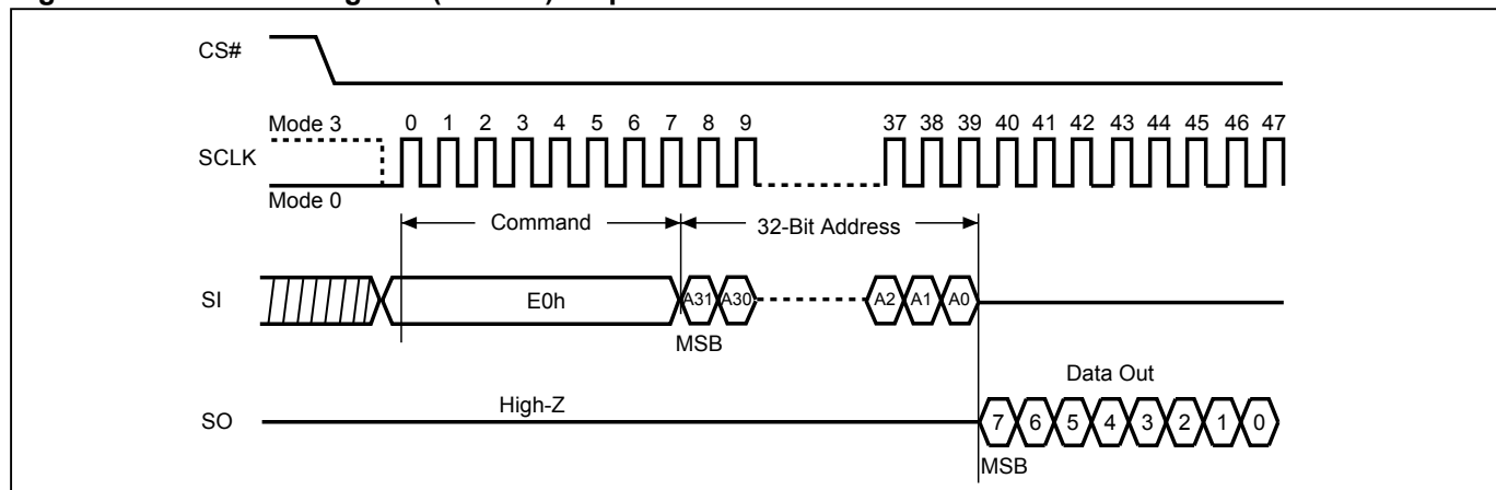
Figure 76. Read DPB Register (RDDPB) Sequence
