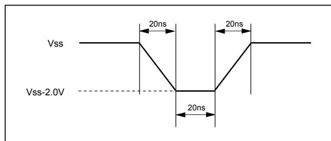
Figure 86. Maximum Negative Overshoot Waveform
