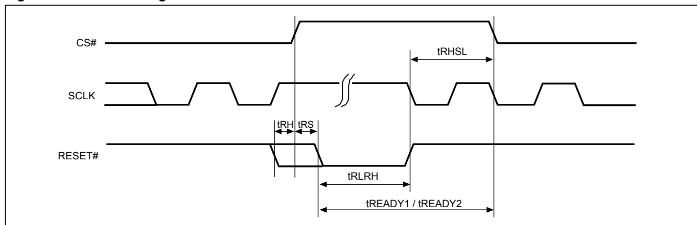
Figure 85. RESET Timing
