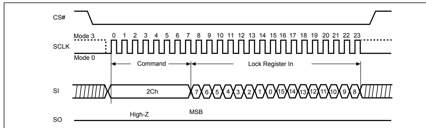
Figure 72. Write Lock Register (WRLR) Sequence
