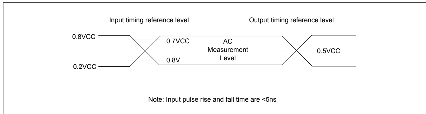
Figure 88. INPUT TEST WAVEFORMS AND MEASUREMENT LEVEL
