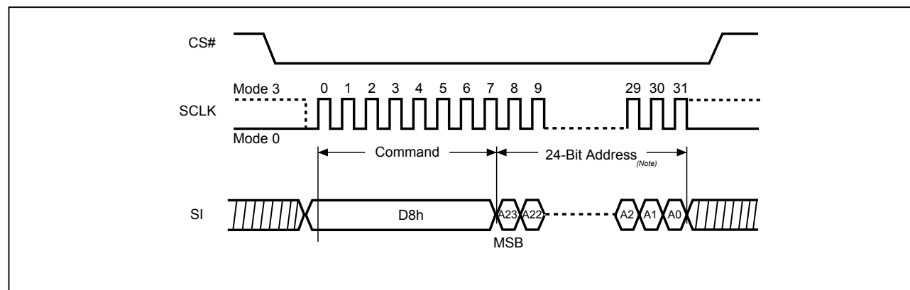
Figure 21. Block Erase (BE) Sequence
