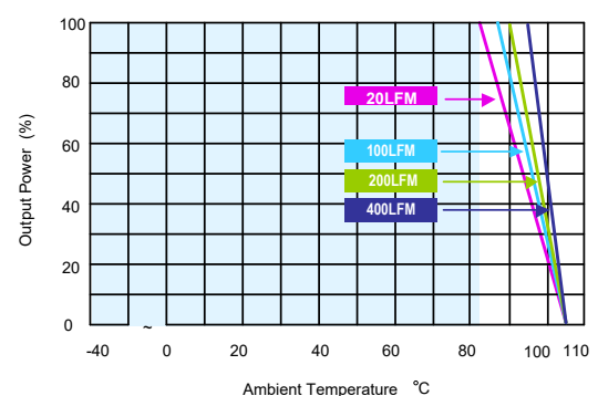
MKZI10-24S05 Derating Curve without Heatsink
