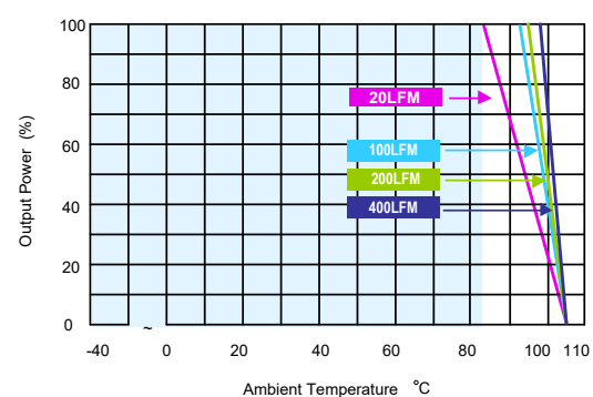
MKZI10-110S05 Derating Curve with Heatsink
