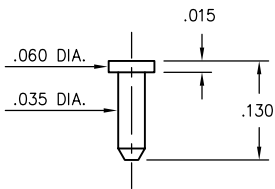
4268-0-00-XX-00-00-33-0 Solder mount in .039 mounting hole
