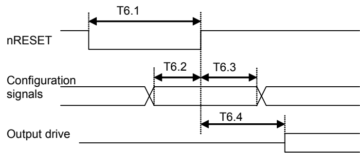
Figure 6.9 Reset Timing
