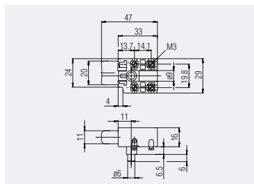
Socket terminal M3 1281.0101
