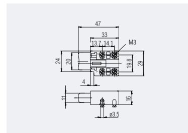
Socket terminal M3 1281.0201
