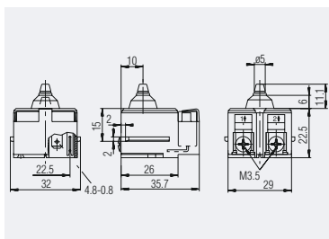
Quick-connect terminal motor side, screw connection mains side with interference suppression capacitor 1246.3101
