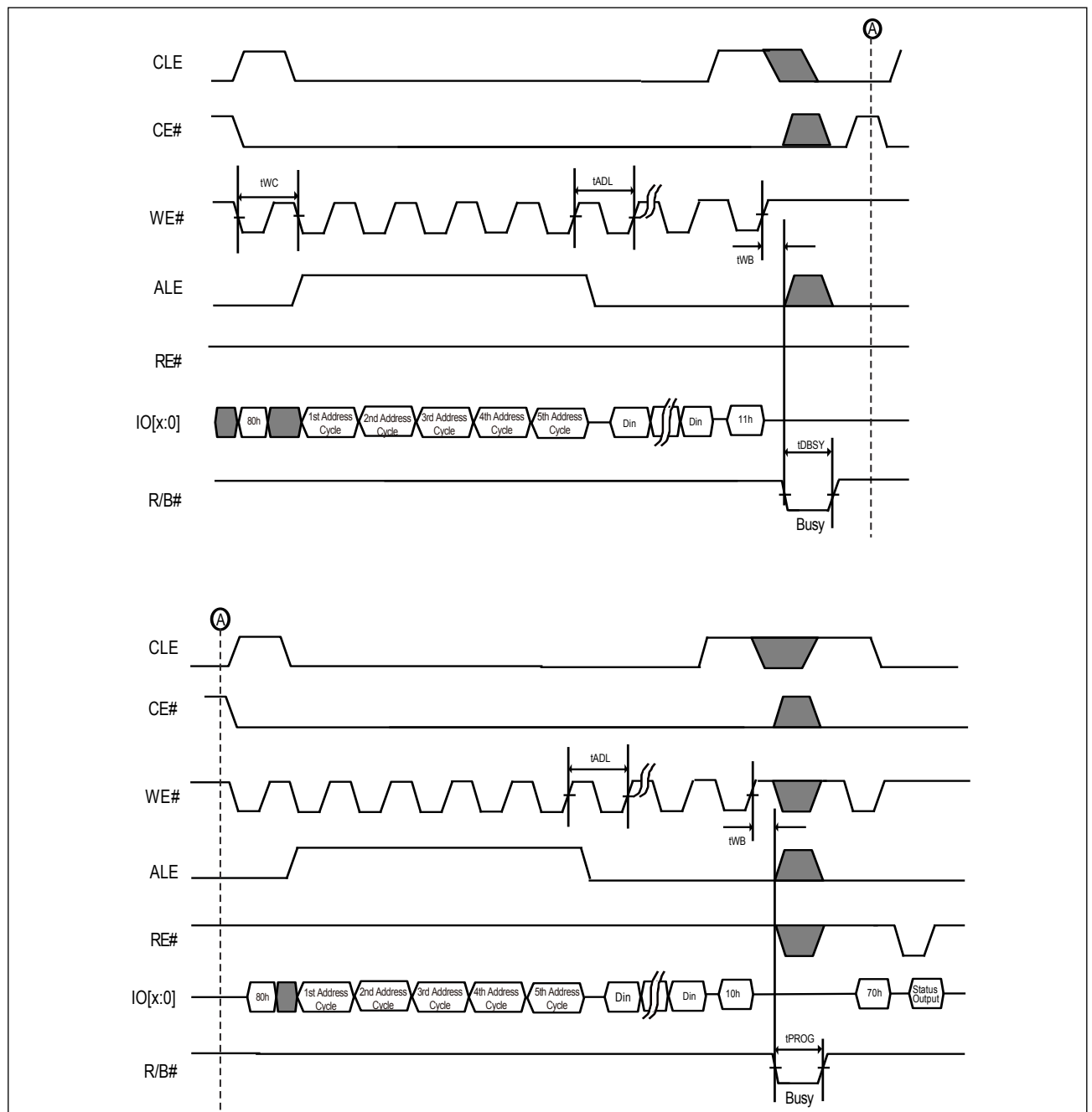
Figure 33-1. AC Waveforms for Two-plane Program (ONFI)
