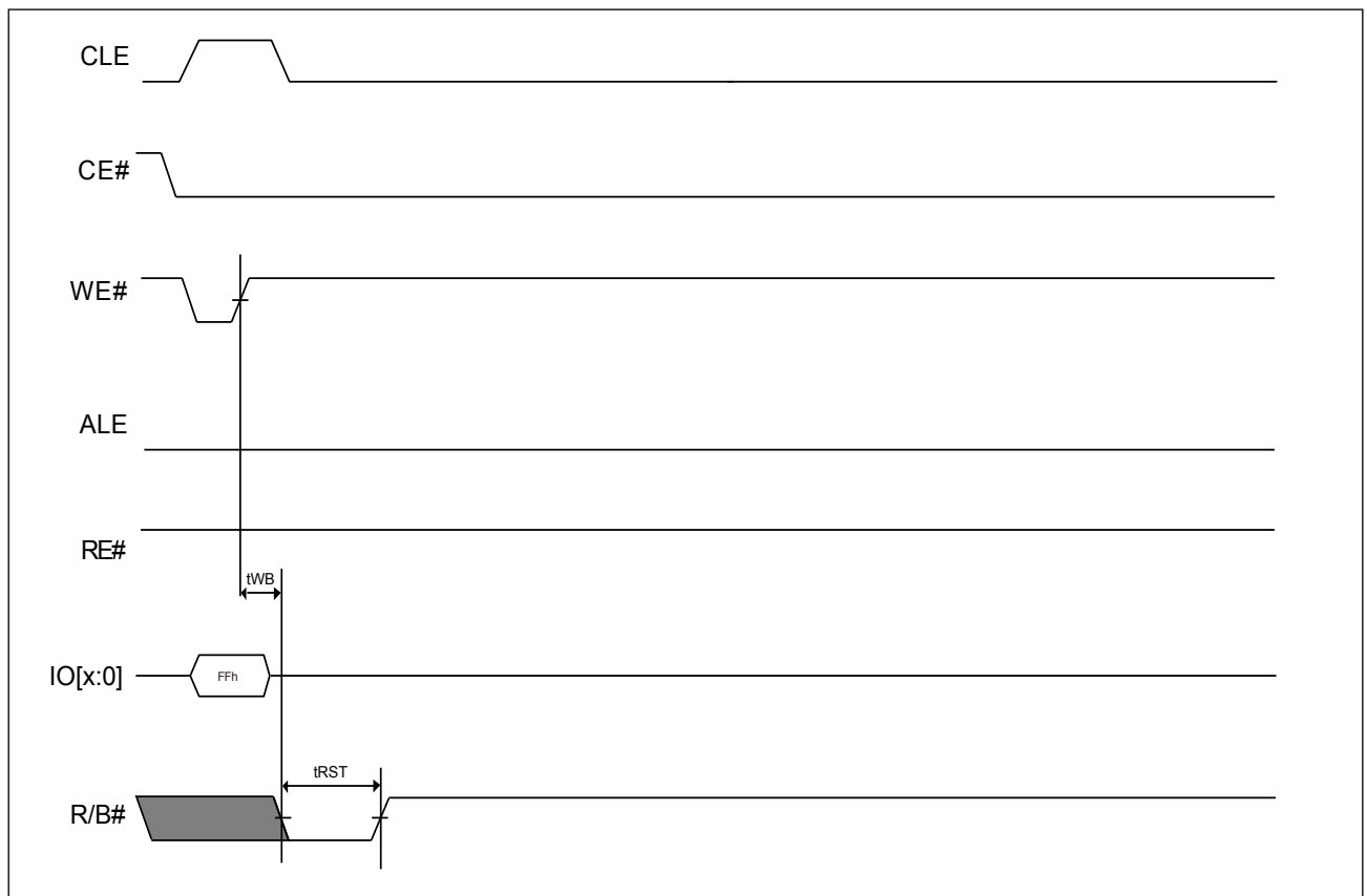
Figure 21. AC waveforms for Reset Operation
