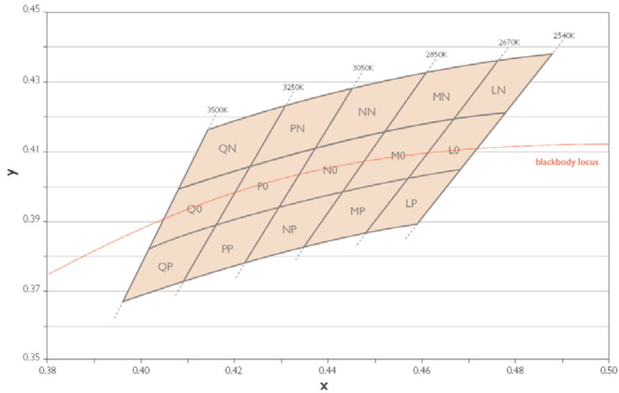
Figure 25: Warm-White Bin Structure.
