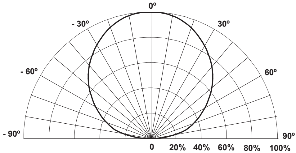
Figure 17b: Typical Polar Radiation Pattern for Cool-White, Neutral-White and Warm-White Lambertian.
