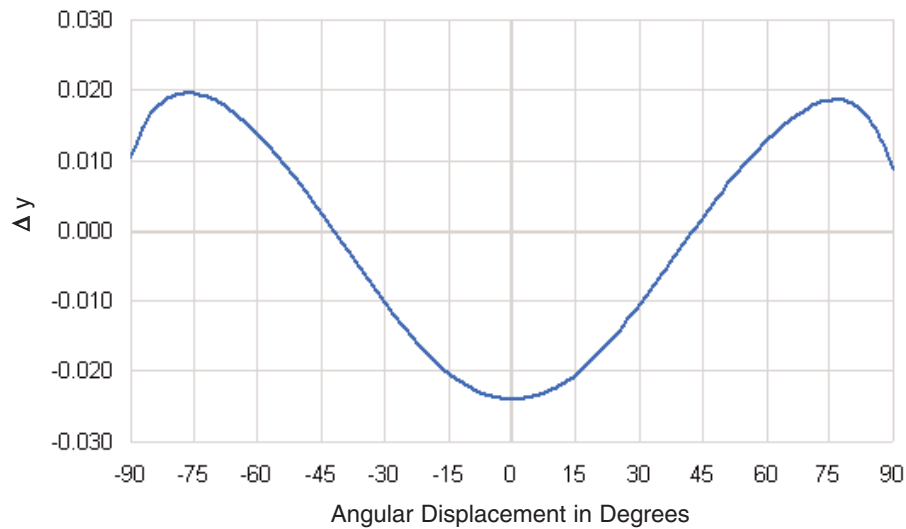
Figure 18b: y coordinate vs. angle for warm-white LUXEON Rebel.
