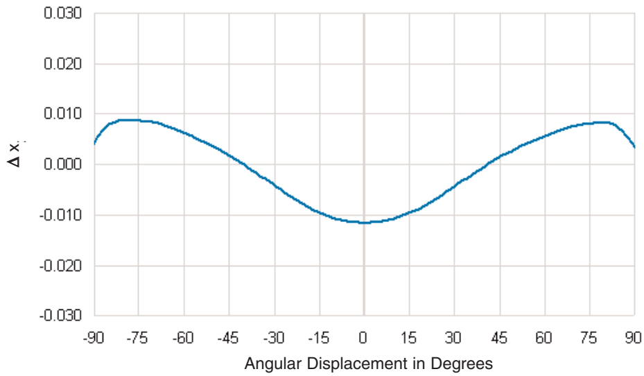
Figure 18a: x coordinate vs. angle for warm-white LUXEON Rebel.
