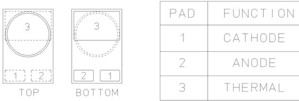
Figure 2. Pad Configuration.
