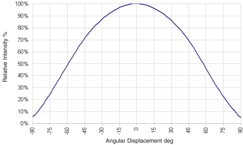
Figure 17a: Typical Representative Spatial Radiation Pattern for Cool-White, Neutral-White and Warm-White Lambertian.
