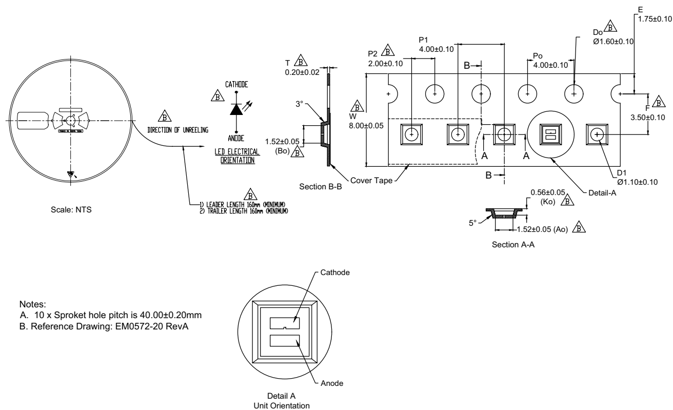
Figure 12. Pocket tape dimensions for LUXEON HL1Z.
