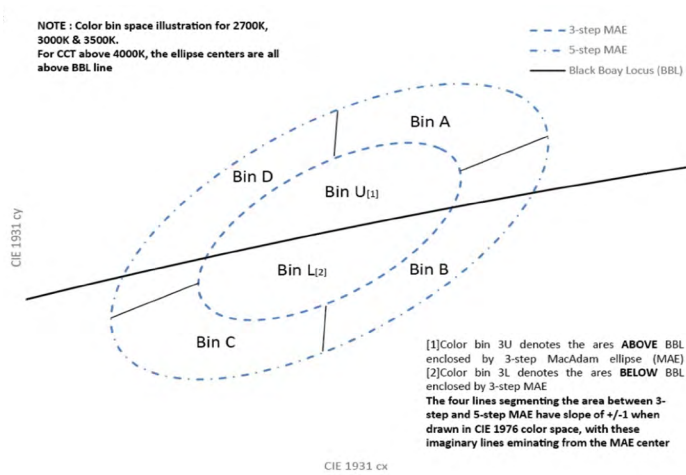
Figure 7. Color space definition for LUXEON HL1Z.
