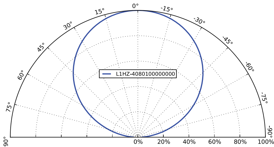
Figure 6. Typical polar radiation pattern for LUXEON HL1Z at 350mA, Tj=85°C.
