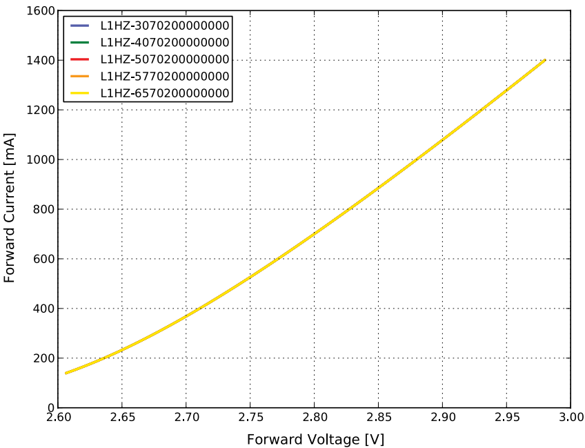
Figure 7. Typical forward current vs. forward voltage for LUXEON HL2Z 70 CRI at T_j=85^{\circ}\text{C} .
