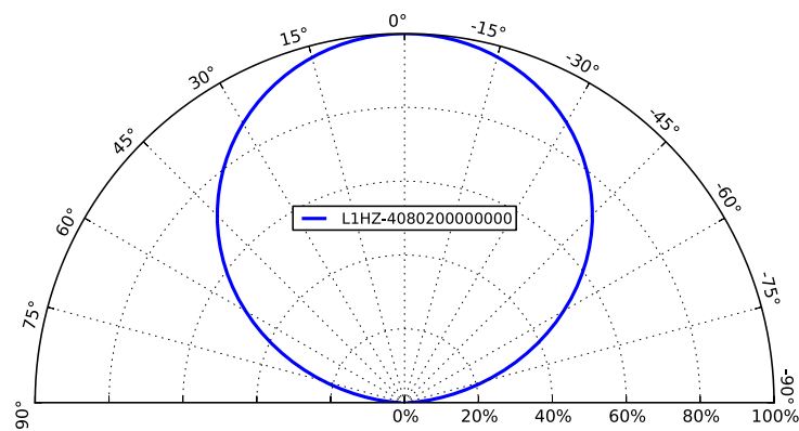
Figure 10. Typical polar radiation pattern for LUXEON HL2Z at 700mA, T_j=85^{\circ}\text{C} .
