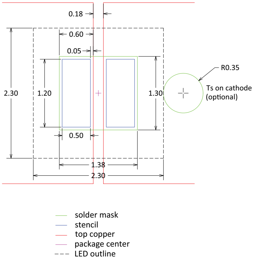
Figure 15. Recommended PCB solder pad layout for LUXEON HL2Z.
