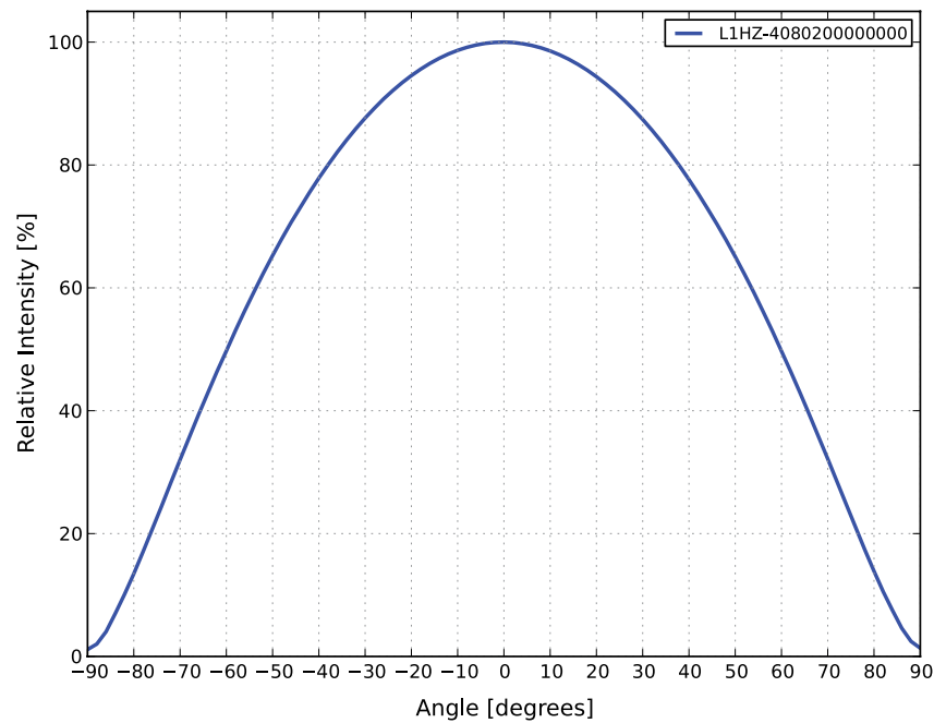
Figure 9. Typical radiation pattern for LUXEON HL2Z at 700mA, T_j=85^{\circ}\text{C} .
