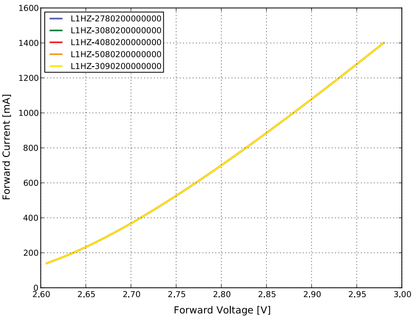
Figure 8. Typical forward current vs. forward voltage for LUXEON HL2Z 80 & 90 CRI at T_j=85^{\circ}\text{C} .
