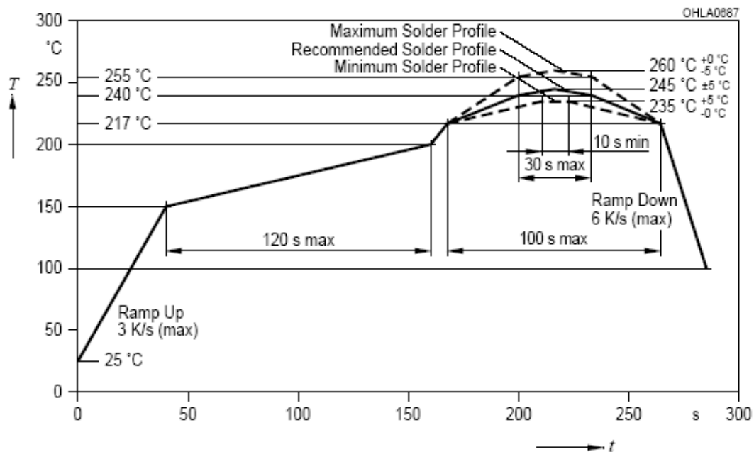
R-Reflow Soldering Profile for lead free soldering (Acc. to J-STD-020D)
