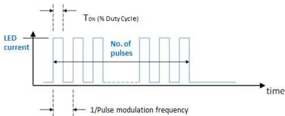
Figure 6.4.1 : LED settings parameters.
