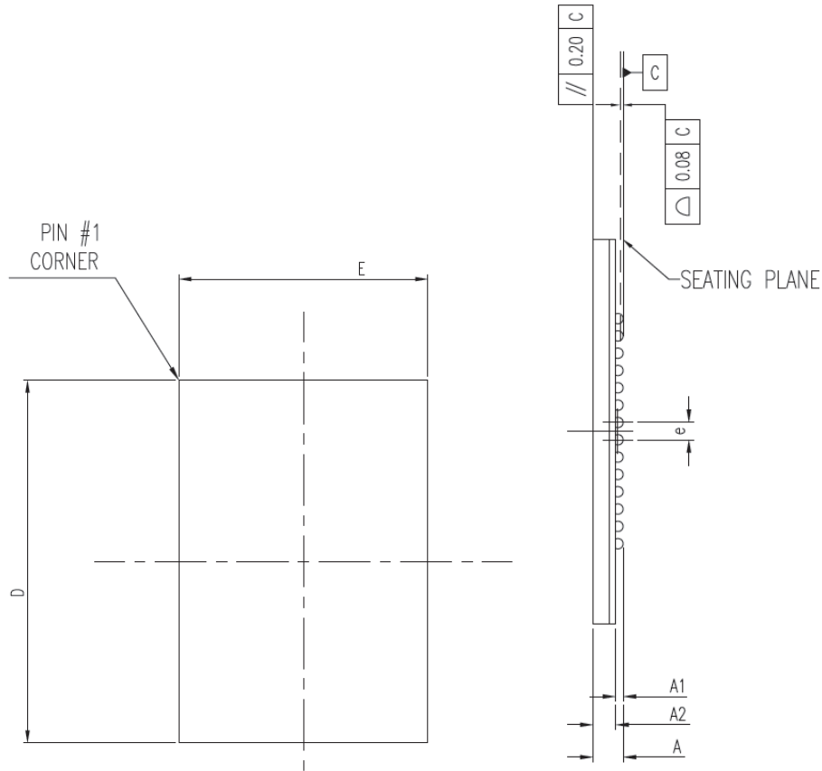
Figure 2 – Package Dimensions
