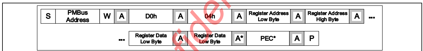
Figure 60 MFR_REG_ACCESS (Write)
