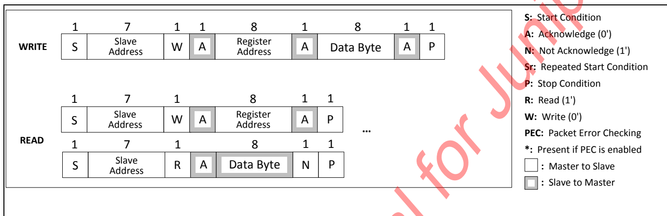
Figure 51 I2C Format
