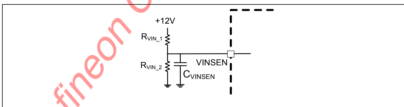
Figure 11 VINSEN Resistor Divider Network
