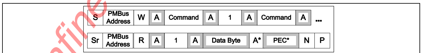
Figure 62 Block Read Process Call
