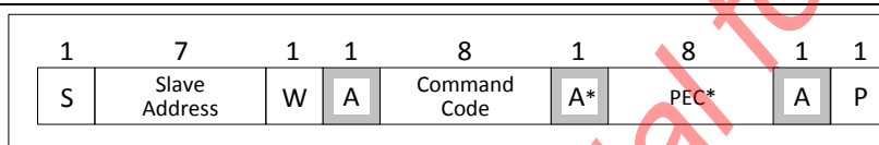
Figure 53 PMBus Send Byte
