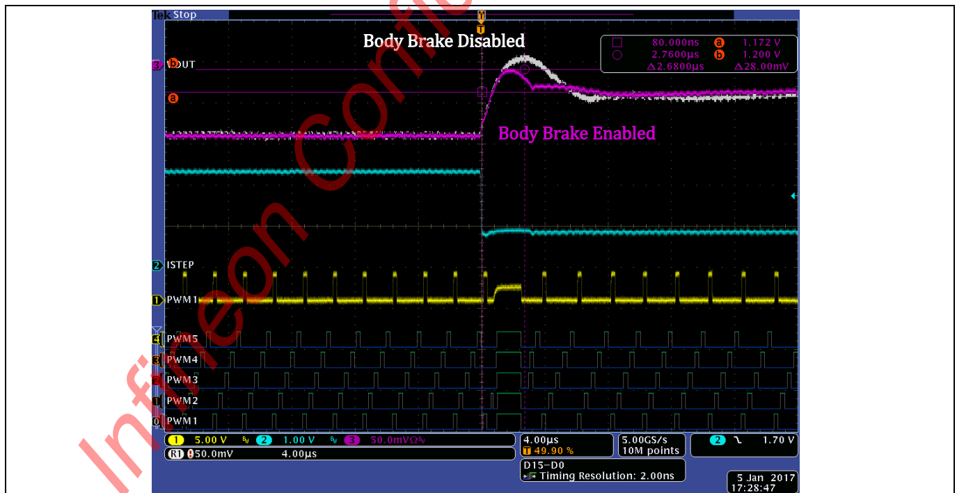
Figure 27 Body Braking during Load Release
