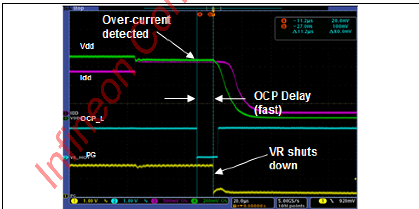
Figure 48 OCP_L (VR_HOT) assertion with OCP_spike (Fast) threshold. OCP delay action (11 \mu s)
