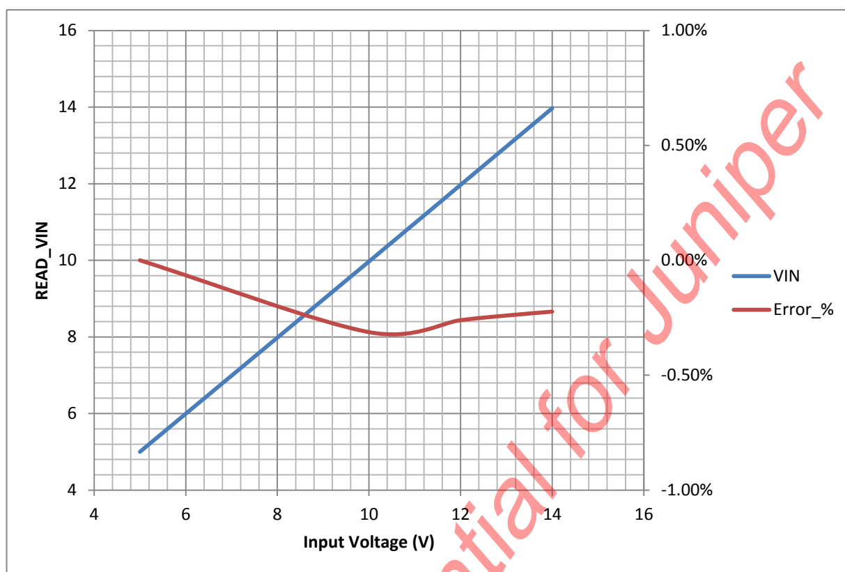
Figure 42 Input Voltage Measurement
