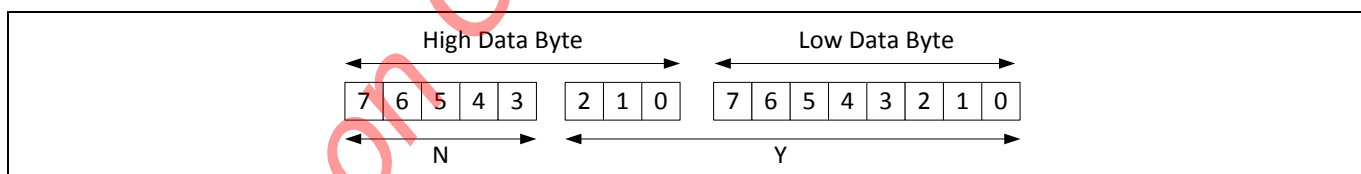
Figure 64 11-bit Linear Data Format
