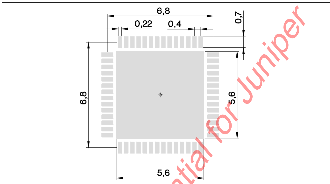
Figure 68 PCB PAD Dimensions
