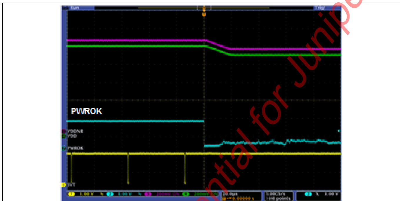
Figure 47 PWR0K De-assertion
