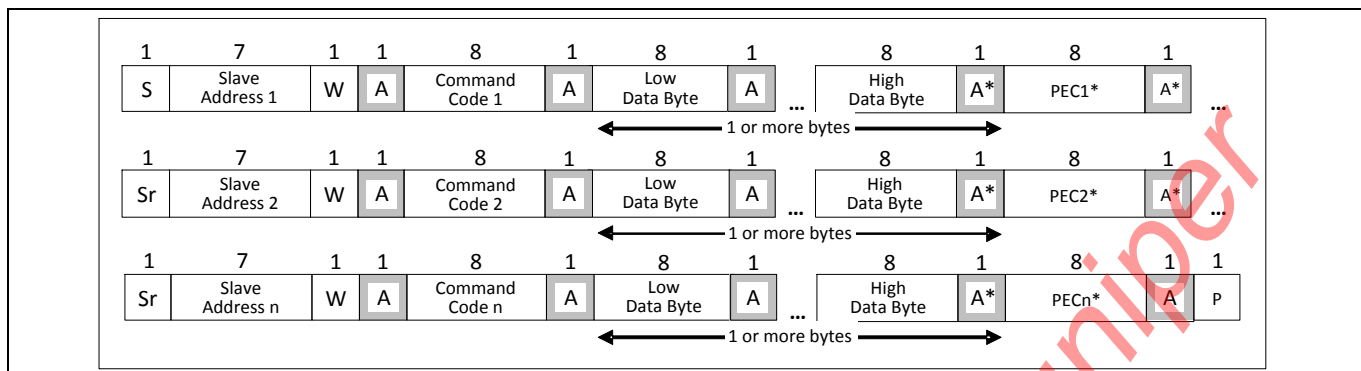
Figure 63 Group Command
