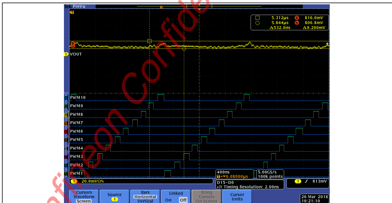
Figure 18 PWM Interleaving for 10 phases
