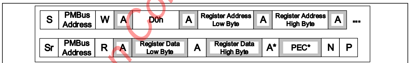
Figure 61 MFR_REG_ACCESS (Read)
