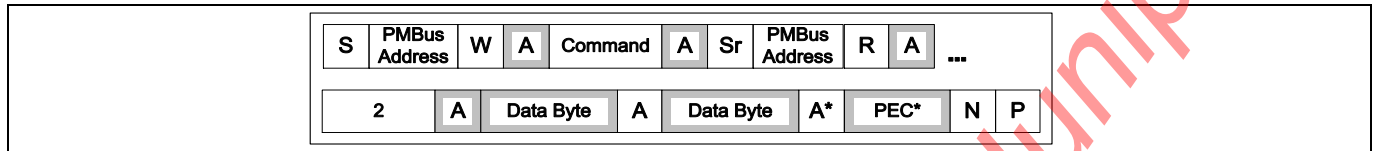
Figure 57 PMBus Block Read with Byte Count = 2
