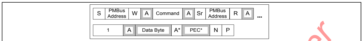
Figure 56 PMBus Block Read with Byte Count = 1
