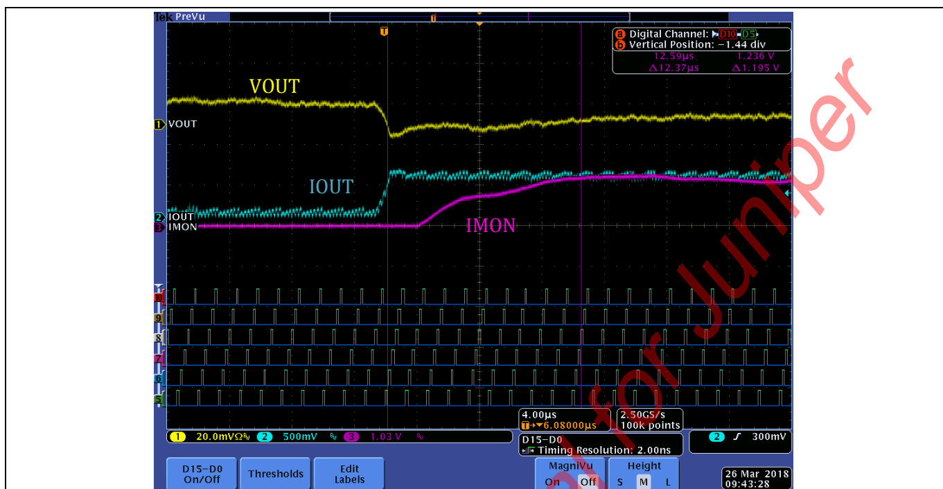
Figure 7 Response time IMON Voltage (V) versus Output Current (A)
