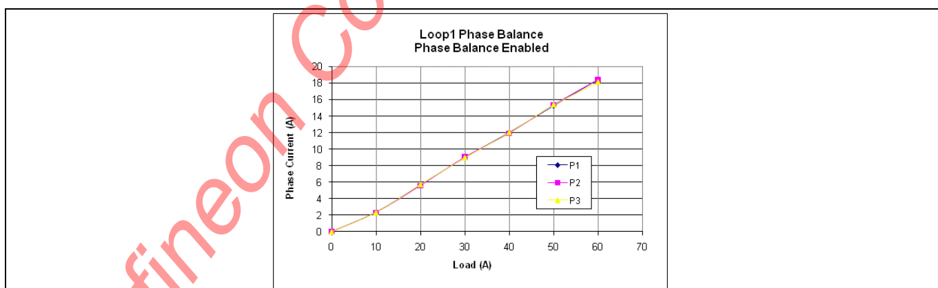
Figure 23 Typical Phase Current Balance (3-Phases enabled)
