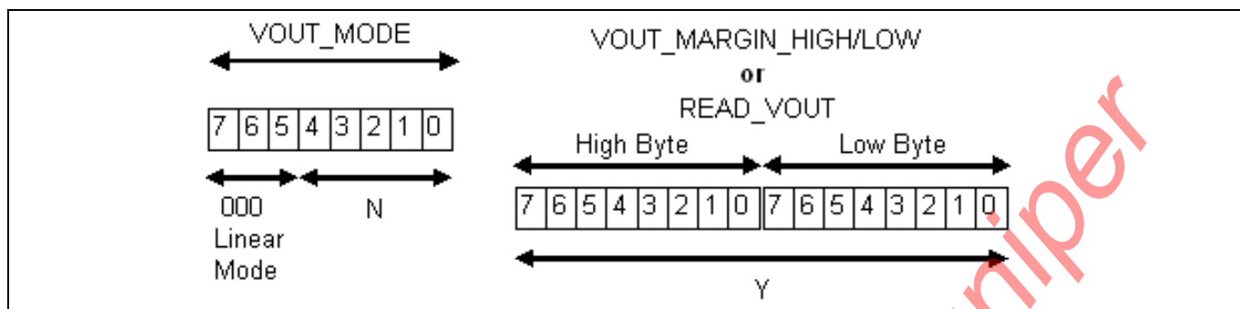
Figure 65 16-bit Linear Data Format
