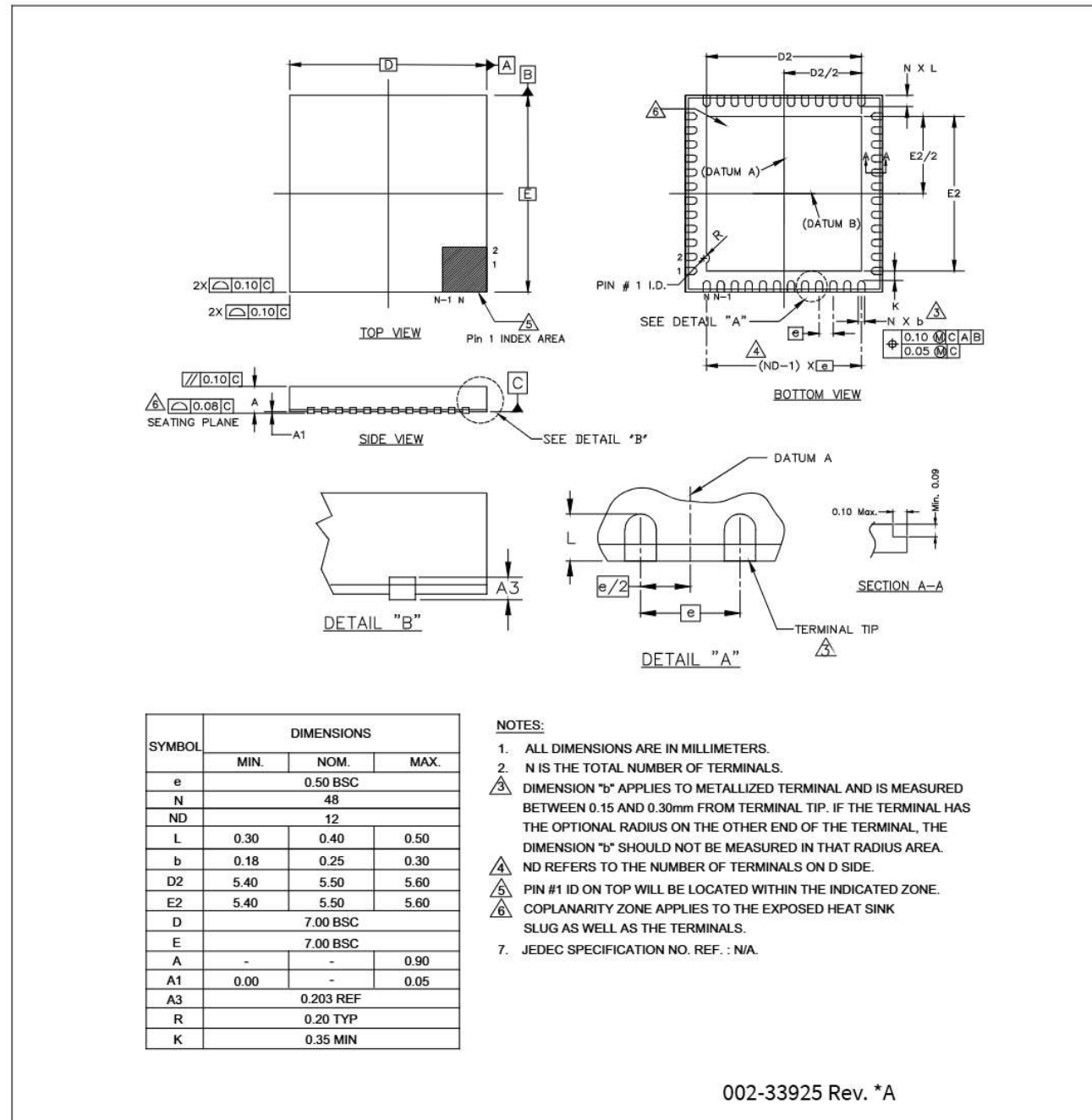
Figure 9 48-pin QFN ((7.0 × 7.0 × 0.9 mm) LV48G 5.5 × 5.5 mm E-Pad (Wettable flank)) package outline, 002-33925
