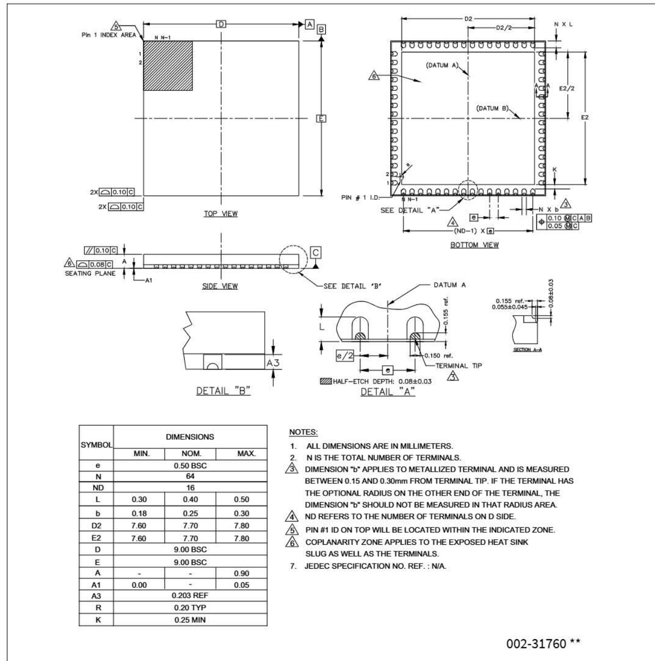
Figure 8 64-pin QFN (9 x 9 x 0.9 mm) LV64A 7.70 x 7.70 mm E-Pad (Sawn)) package outline (PG-VQFN-64), 002-31760
