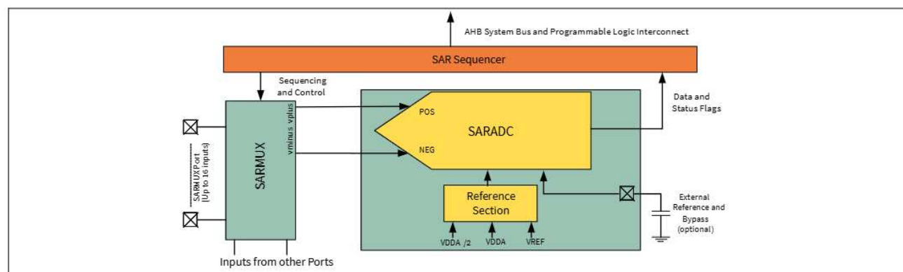
Figure 3 SAR ADC
