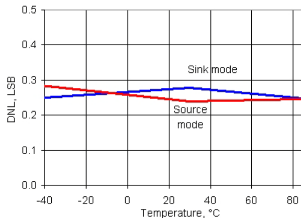
Figure 11-40. IDAC DNL vs Temperature, Range = 255 \mu A, High speed mode
