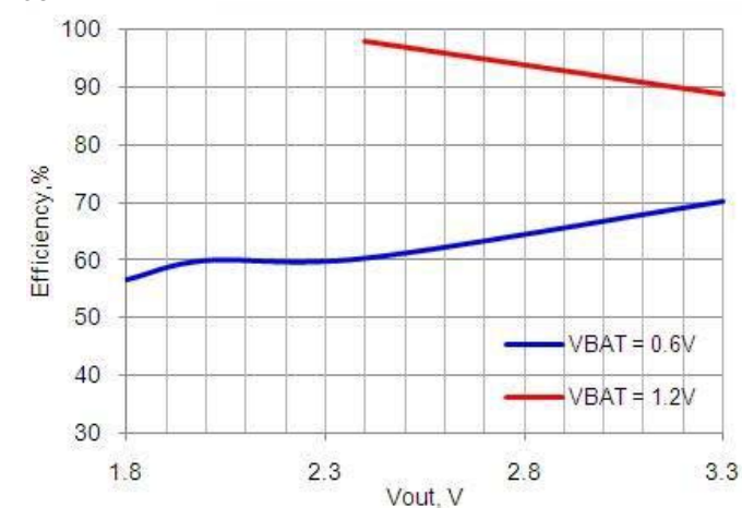
Figure 11-10. Efficiency vs V_{\text{OUT}}
