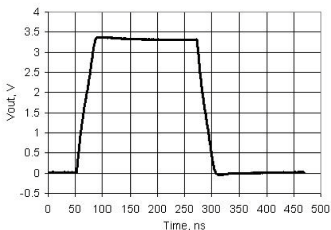
Figure 11-15. GPIO Output Rise and Fall Times, Slow Strong Mode, V_{DDIO} = 3.3 V, 25 pF Load
