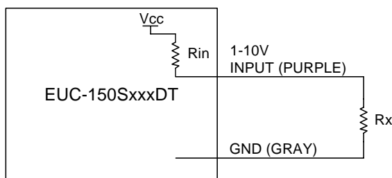
Implementation 2: External resistor
