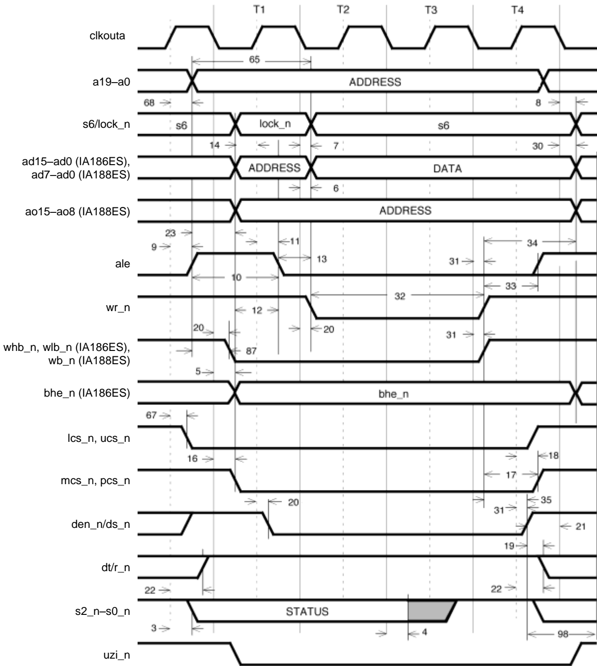
Figure 14. Write Cycle
