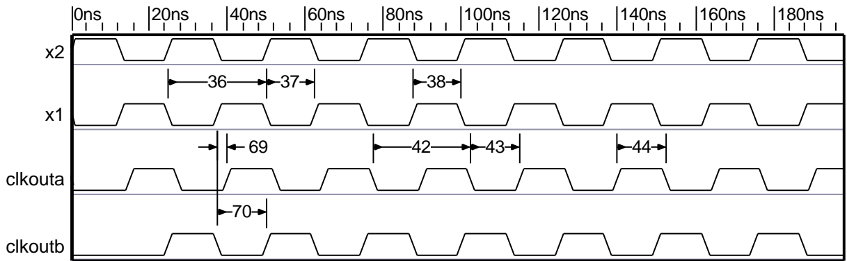
Figure 21. Clock—Active Mode
