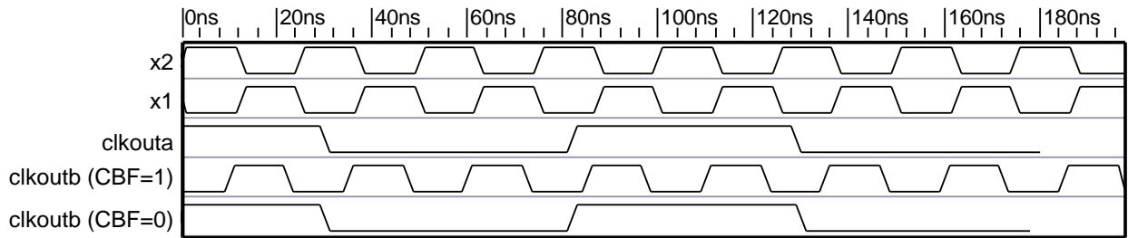
Figure 22. Clock—Power-Save Mode
