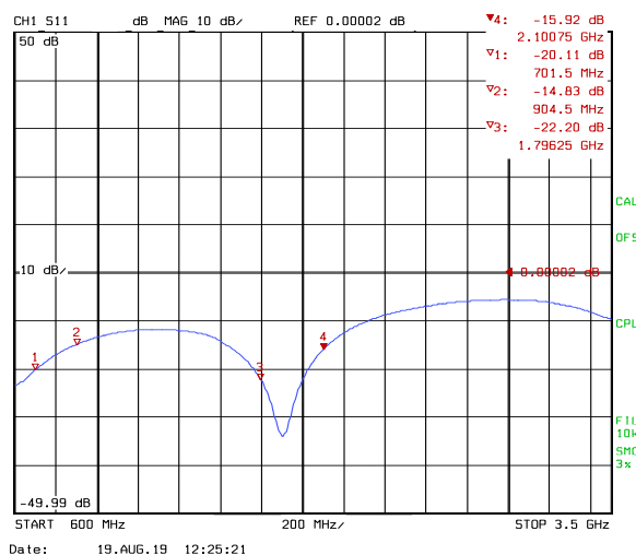
Figure 19: S11 MAIN antenna input return loss transmit direction (with old socket)
