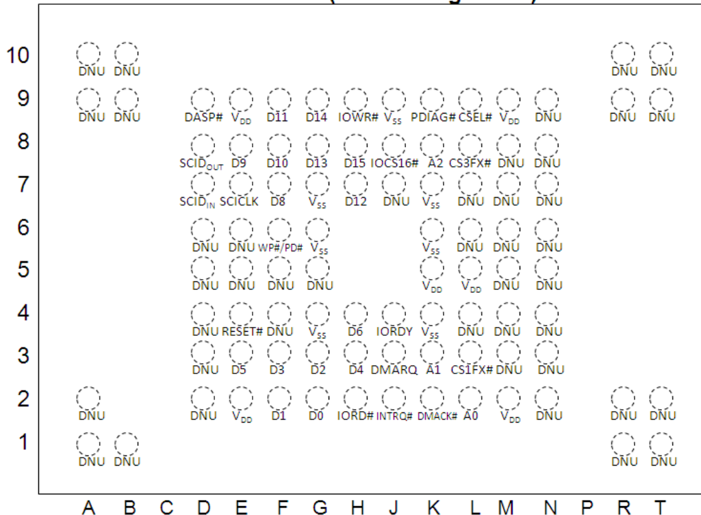
Figure 2: Pin Assignments for 91-Ball LPGA
