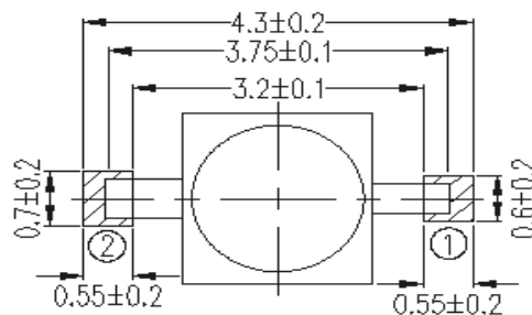
Recommend Soldering Pad
