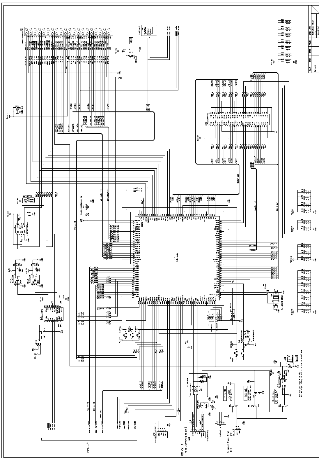
Figure 6-1: S5U13U11P00C100 Schematic Diagram (1 of 2)
