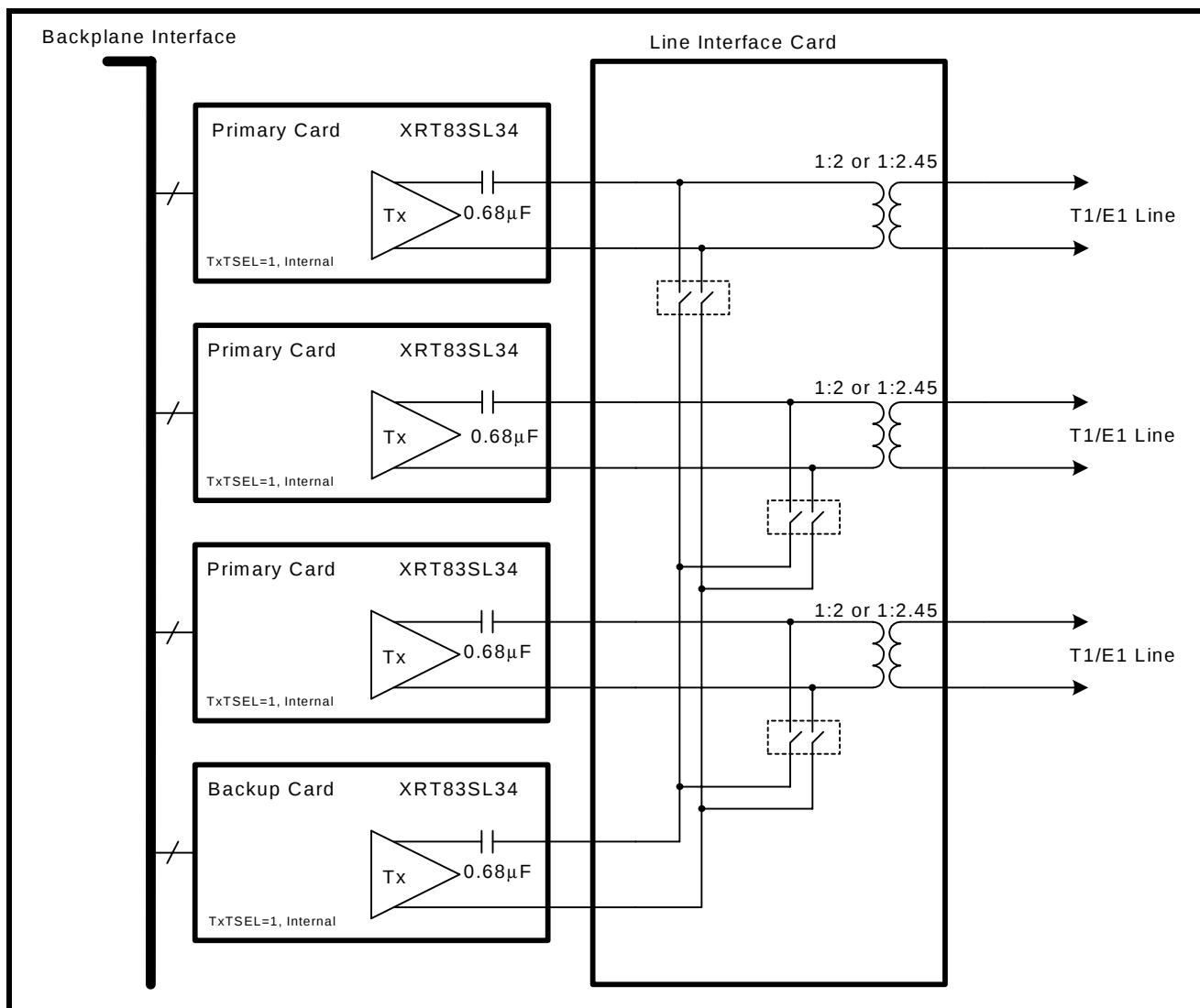
FIGURE 16. SIMPLIFIED BLOCK DIAGRAM - TRANSMIT SECTION FOR N+1 REDUNDANCY
