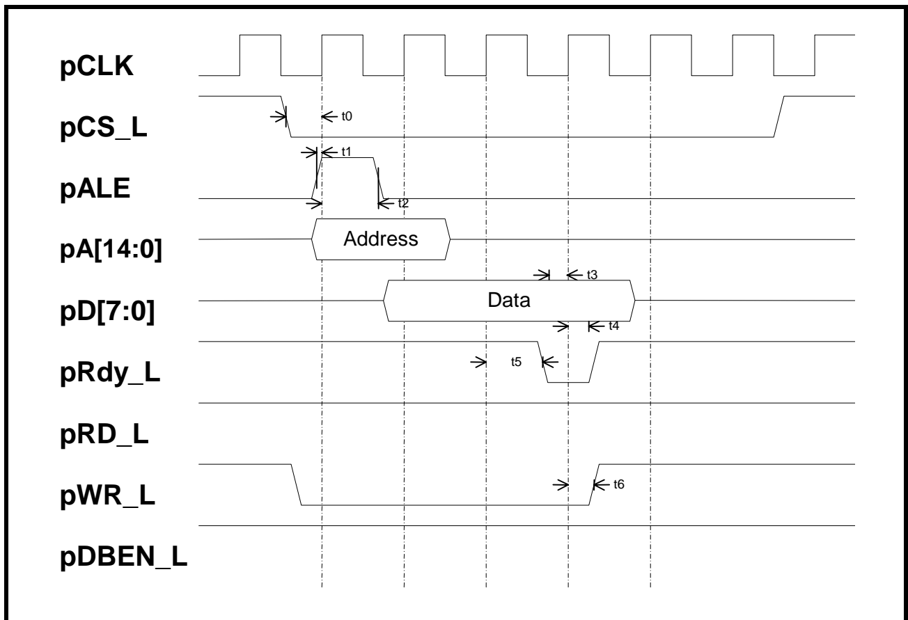
FIGURE 12. SYNCHRONOUS MODE 4 - IDT 3051/52 INTERFACE TIMING (WRITE CYCLE)
