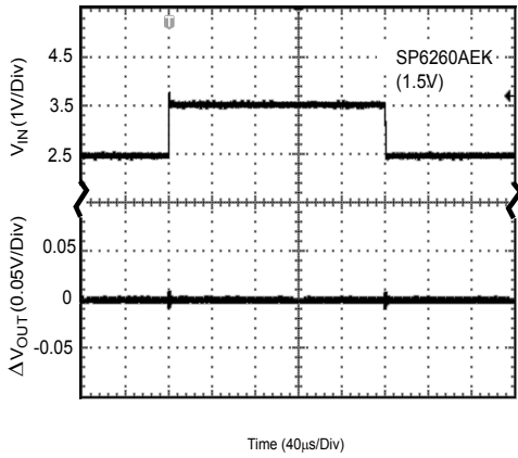
SP6260AEK (1.5V) Line Transient (Conditions: I_{OUT}=30\text{mA} , C_{IN}=1\mu\text{F} , C_{OUT}=1\mu\text{F} )
