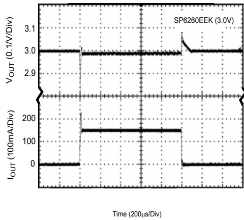
SP6260EEK (3.0V) Load Transient (Conditions: V_{IN}=4\text{V} , C_{IN}=1\mu\text{F} , C_{OUT}=1\mu\text{F} )
