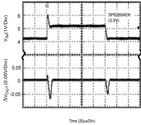
SP6260EEK (3.0V) Line Transient (Conditions: I_{OUT}=30\text{mA} , C_{IN}=1\mu\text{F} , C_{OUT}=1\mu\text{F} )
