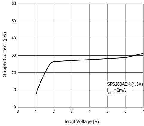
Supply Current vs. Input Voltage SP6260AEK (1.5V)
