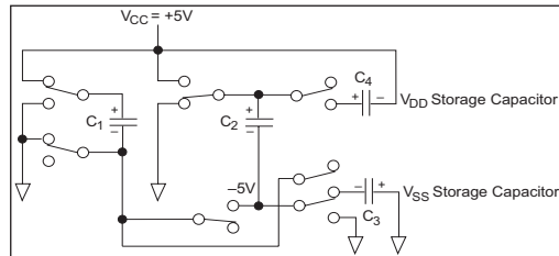
Figure 15b. Charge Pump Phase 2 for ±5V.
