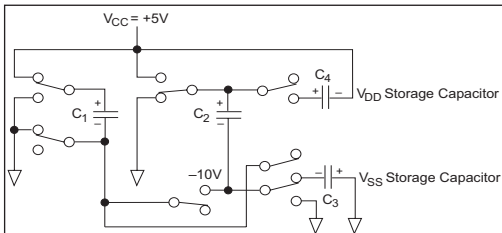
Figure 15a. Charge Pump Phase 2 for ±10V.
