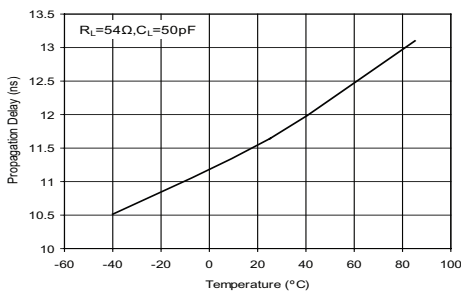
Driver Average Propagation Delay vs Temperature (SP3086-SP3088)
