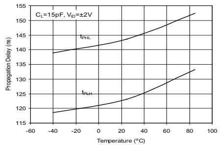
Receiver Propagation Delay vs Temperature (SP3083-SP3085)
