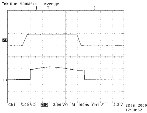
Receiver Propagation Delay (SP3083-SP3085)
