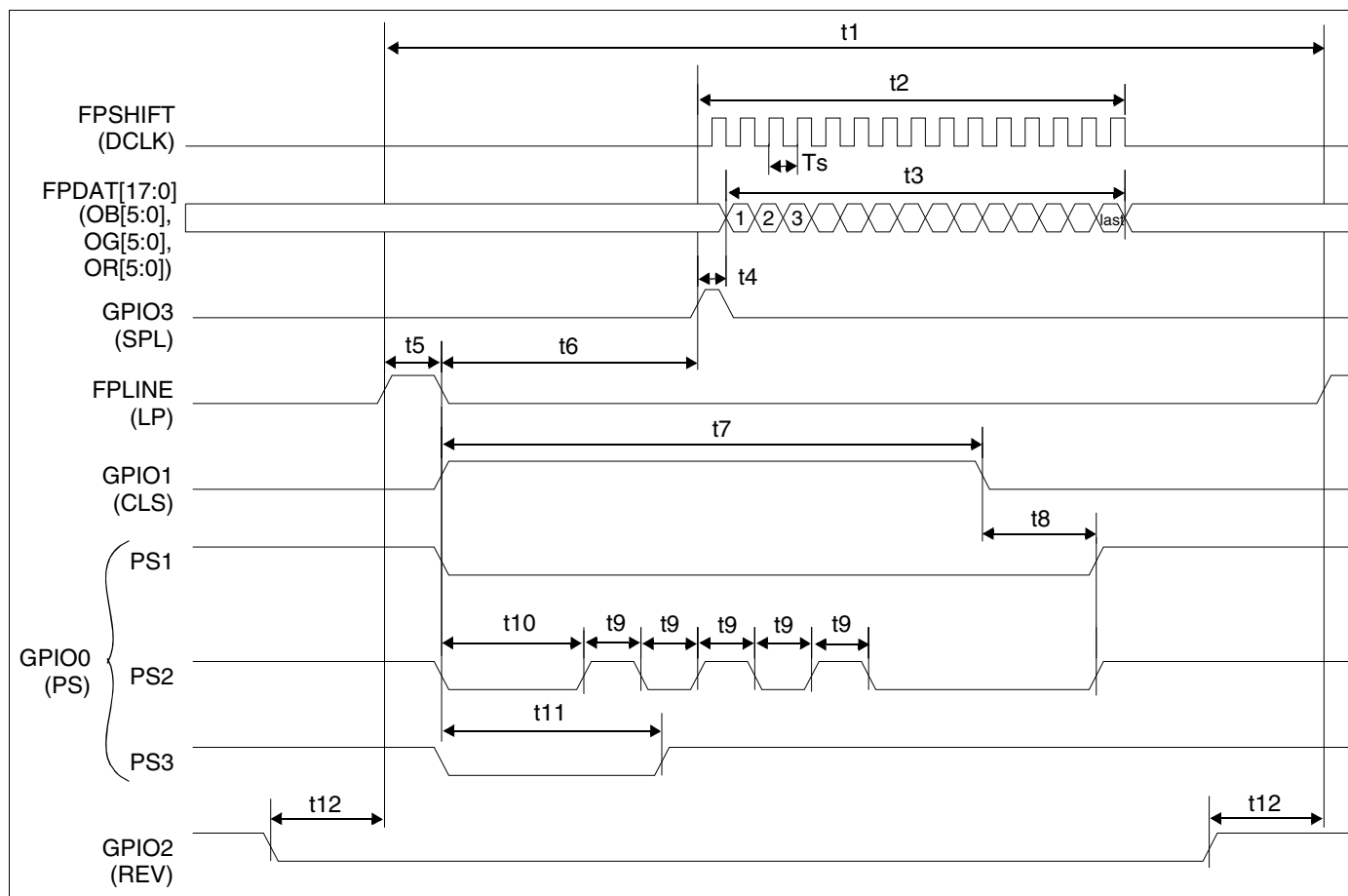
Figure 6-31: Sharp HR-TFT Panel Horizontal Timing
