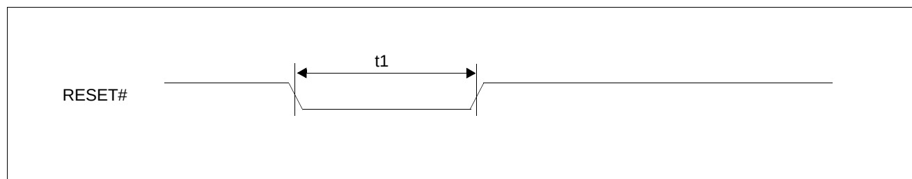
Figure 6-2 S1D13A05 RESET# Timing
