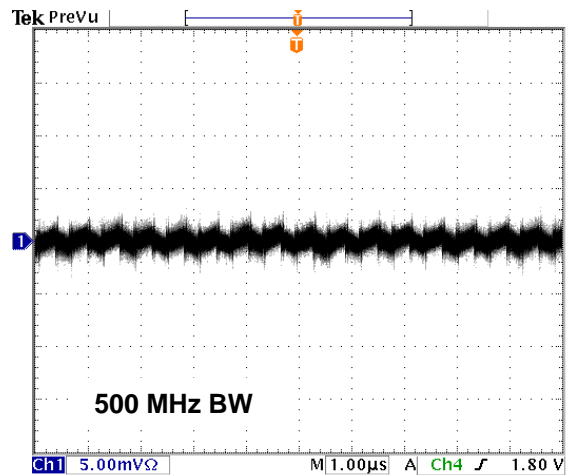
Output Ripple: AVIN = 3.3V, VDDQ = 1.5V, VOUT = VDDQ*0.5, I out = 8A, C IN = 2x47μF (0805), C OUT = 4x100μF (1206)
