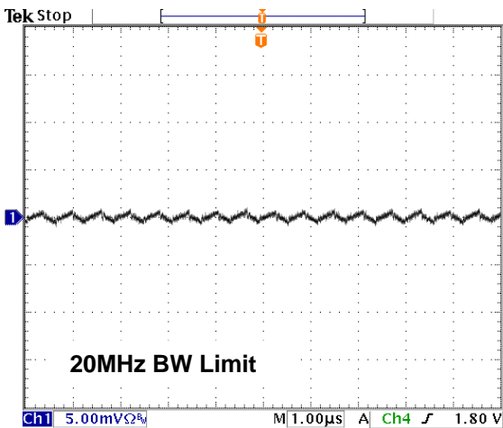
Output Ripple: AVIN = 3.3V, VDDQ = 1.5V, VOUT = VDDQ*0.5, I out = 8A, C IN = 2x47μF (0805), C OUT = 4x100μF (1206)
