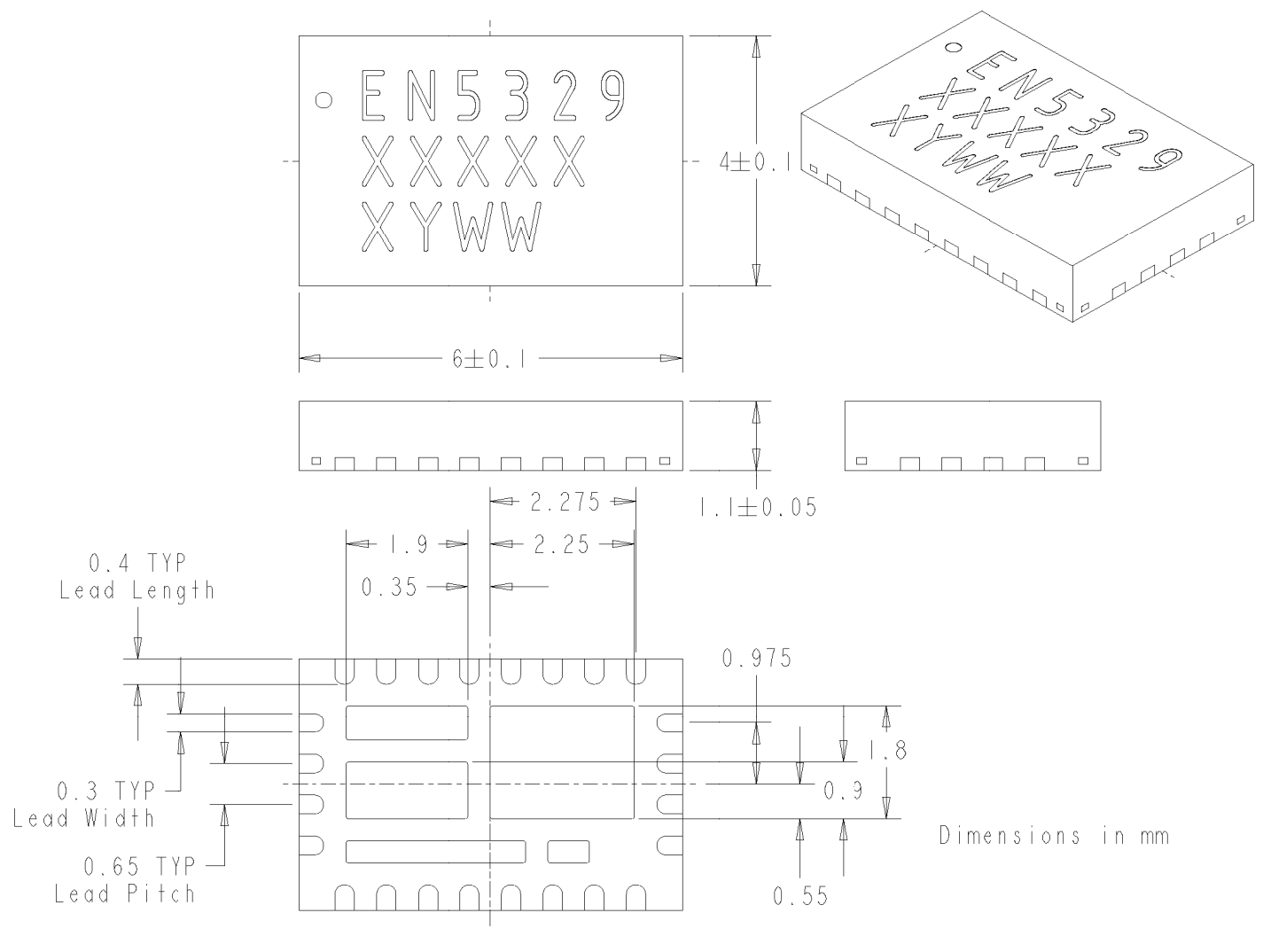
Figure 11. EN5329QI Package Dimensions (Bottom View)
