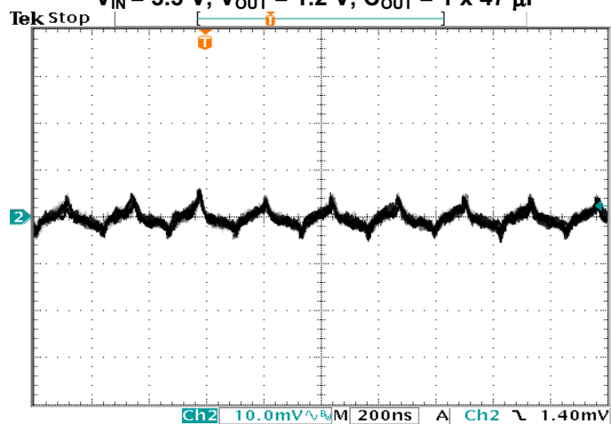
Output Ripple at 2 A Load (CH2: V OUT )
