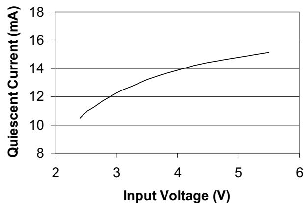
Quiescent Current (Switching) vs. Input Voltage
