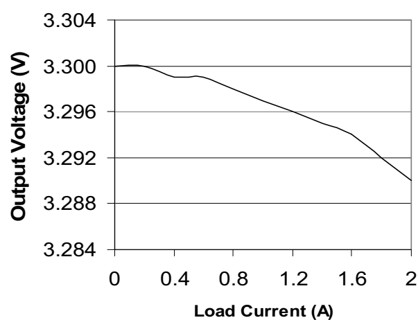
Load Regulation (Vin = 5 V)
