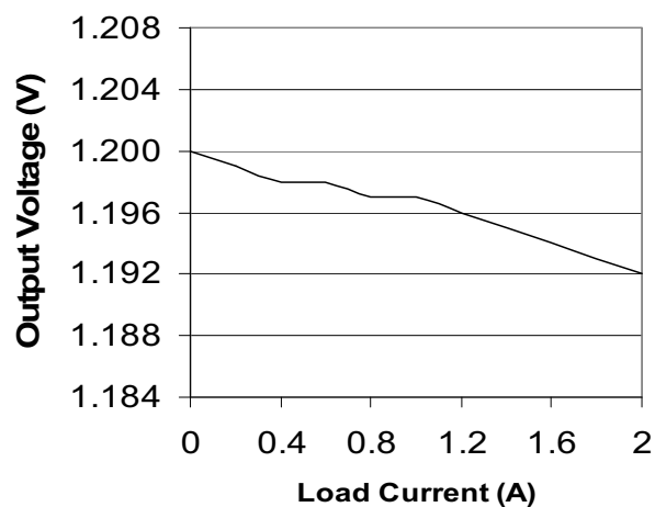
Load Regulation (Vin = 5 V)
