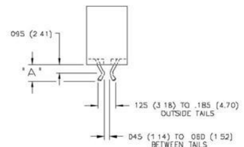
CONTACT CODE 556
