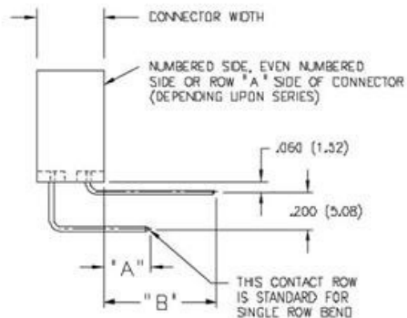
CONTACT CODE 558
