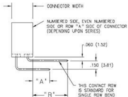
CONTACT CODE 559
