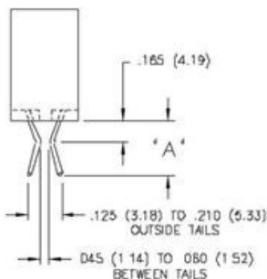
CONTACT CODE 560
