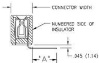
CONTACT CODE 557
