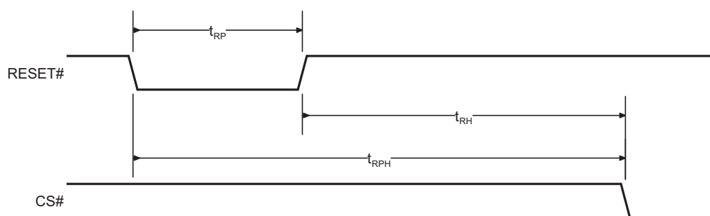
Figure 22. Hardware Reset Timing Diagram
