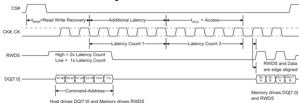
Figure 2. Read Transaction
