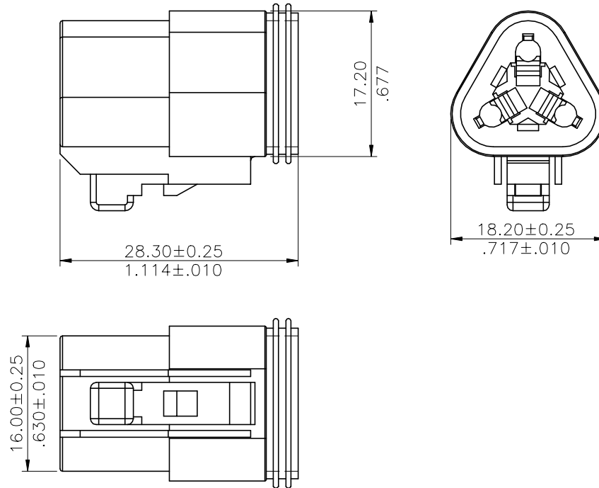
HOUSING
