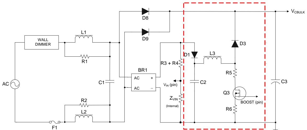
Figure 7. Chopper Circuit
