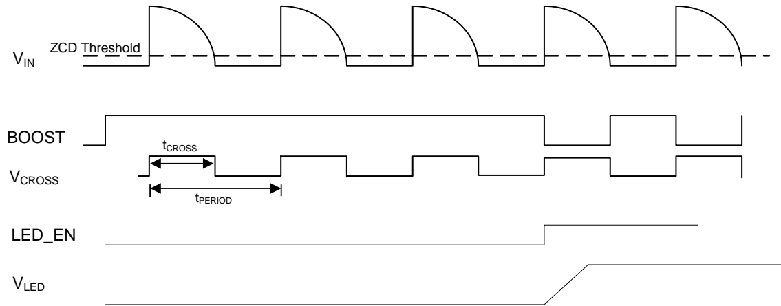
Figure 4. Dimmer Detection
