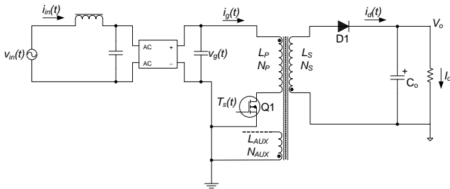
Figure 10. Simplified Flyback Converter
