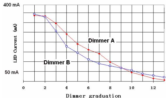
Figure 22. Dimming Curve
