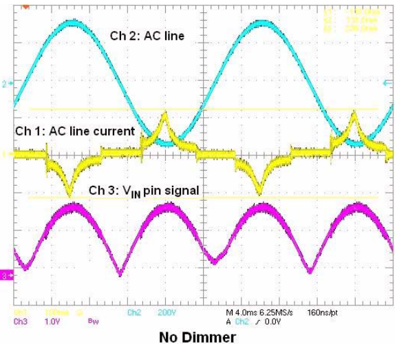
Figure 21. Inrush and AC Peak Current (No Dimmer)
