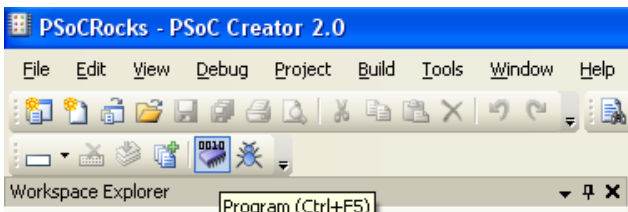
Figure 4-4. Program
