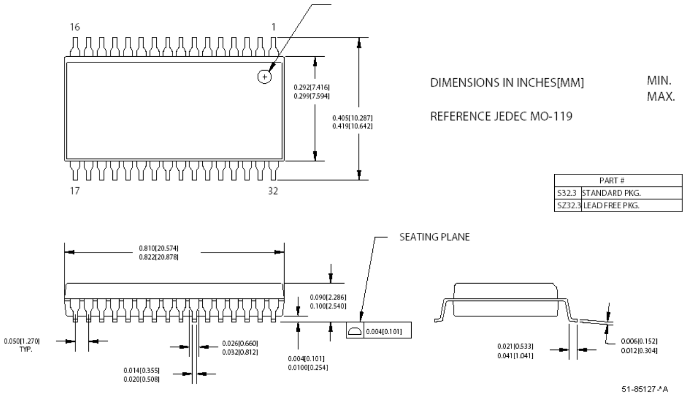
Figure 18. 32-Pin SOIC (51-85127)
