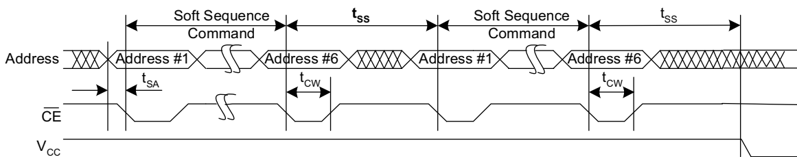
Figure 15. Soft Sequence Processing [28, 29]
